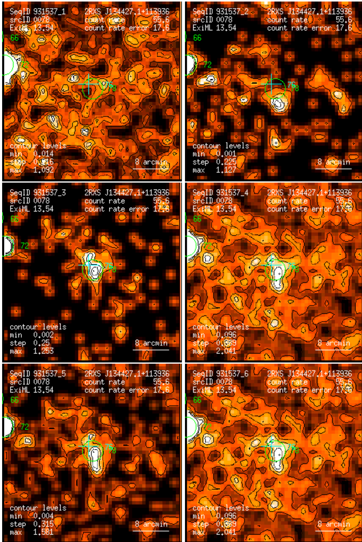
Figure 78: RASS 931537: detection 0078: band rate images, Gaussian filter: (1) PSPC channels 11 – 41, (2) 52 – 90, (3) 91 – 201, (4) 11 – 235, (5) 52 – 201, (6) 11 – 201. Broad band rates in counts/ks. Band rate contour levels in counts/ks/arcmin 2 .
