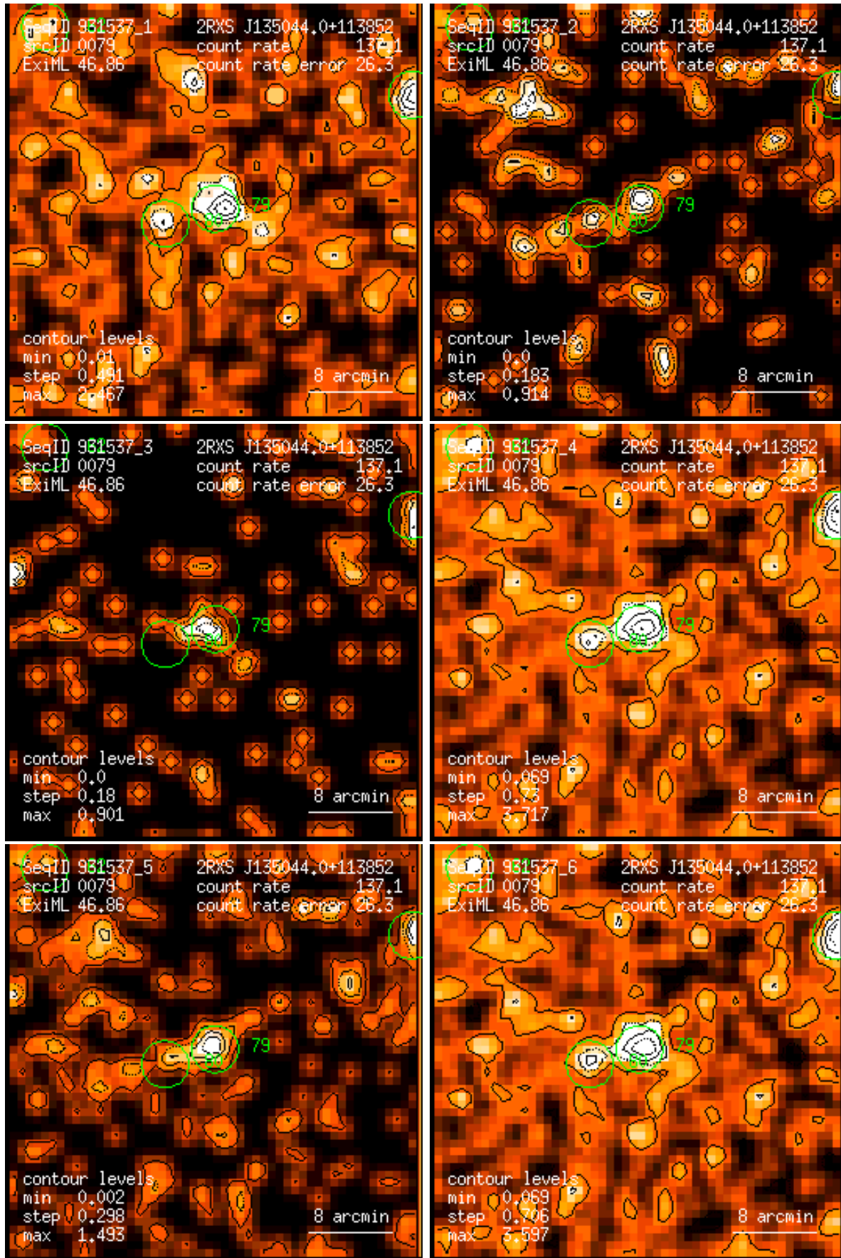
Figure 79: RASS 931537: detection 0079: band rate images, Gaussian filter: (1) PSPC channels 11 – 41, (2) 52 – 90, (3) 91 – 201, (4) 11 – 235, (5) 52 – 201, (6) 11 – 201. Broad band rates in counts/ks. Band rate contour levels in counts/ks/arcmin 2 .
