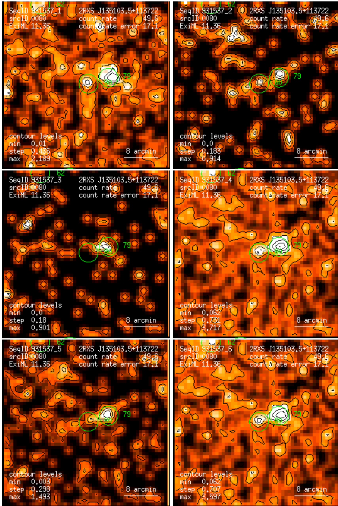
Figure 80: RASS 931537: detection 0080: band rate images, Gaussian filter: (1) PSPC channels 11 – 41, (2) 52 – 90, (3) 91 – 201, (4) 11 – 235, (5) 52 – 201, (6) 11 – 201. Broad band rates in counts/ks. Band rate contour levels in counts/ks/arcmin 2 .
