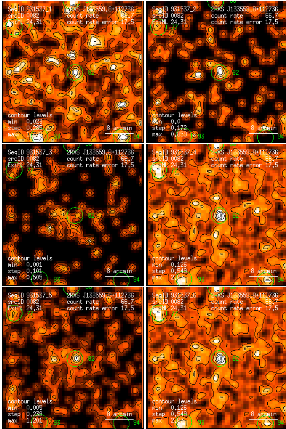
Figure 82: RASS 931537: detection 0082: band rate images, Gaussian filter: (1) PSPC channels 11 – 41, (2) 52 – 90, (3) 91 – 201, (4) 11 – 235, (5) 52 – 201, (6) 11 – 201. Broad band rates in counts/ks. Band rate contour levels in counts/ks/arcmin 2 .
