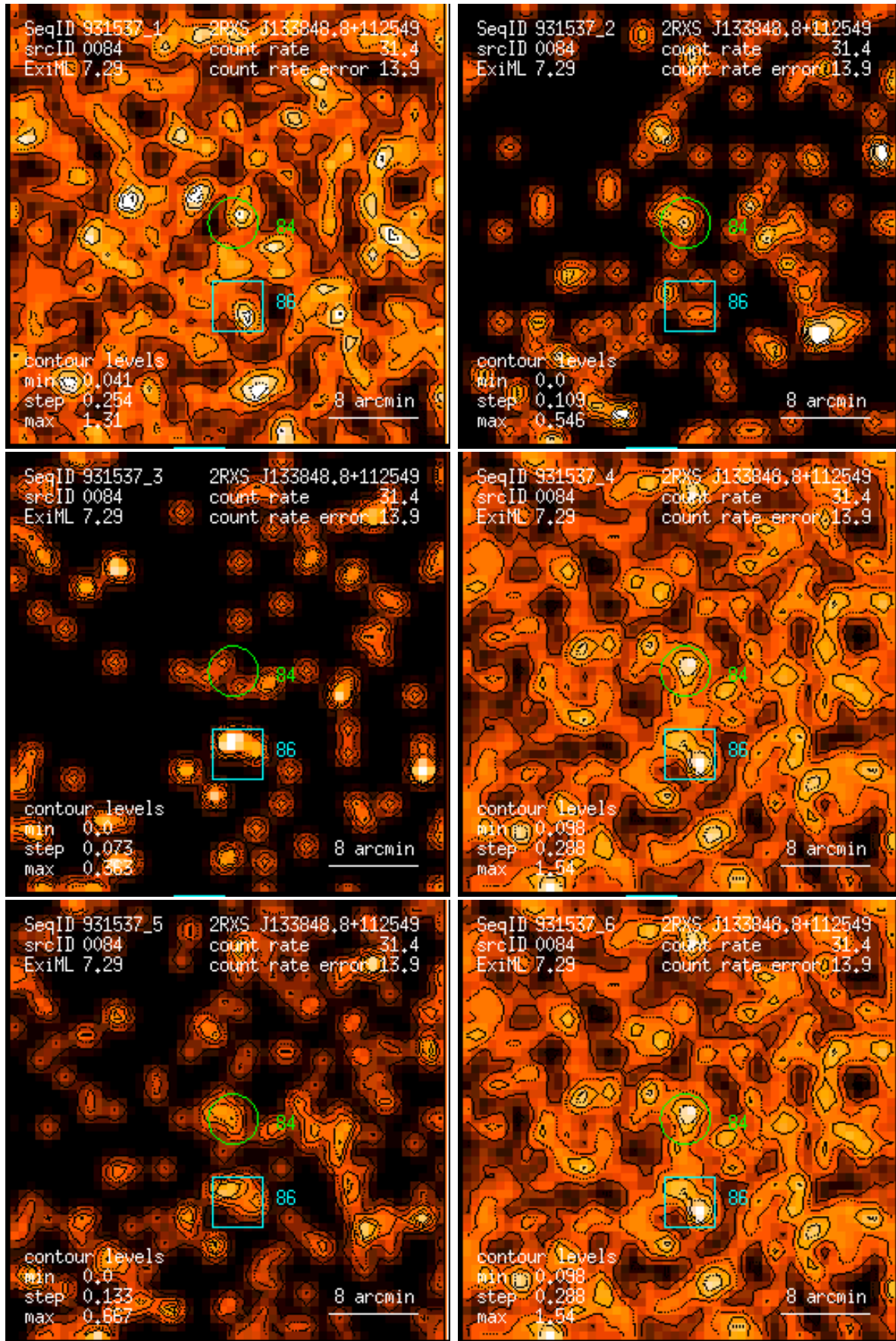
Figure 84: RASS 931537: detection 0084: band rate images, Gaussian filter: (1) PSPC channels 11 – 41, (2) 52 – 90, (3) 91 – 201, (4) 11 – 235, (5) 52 – 201, (6) 11 – 201. Broad band rates in counts/ks. Band rate contour levels in counts/ks/arcmin 2 .
