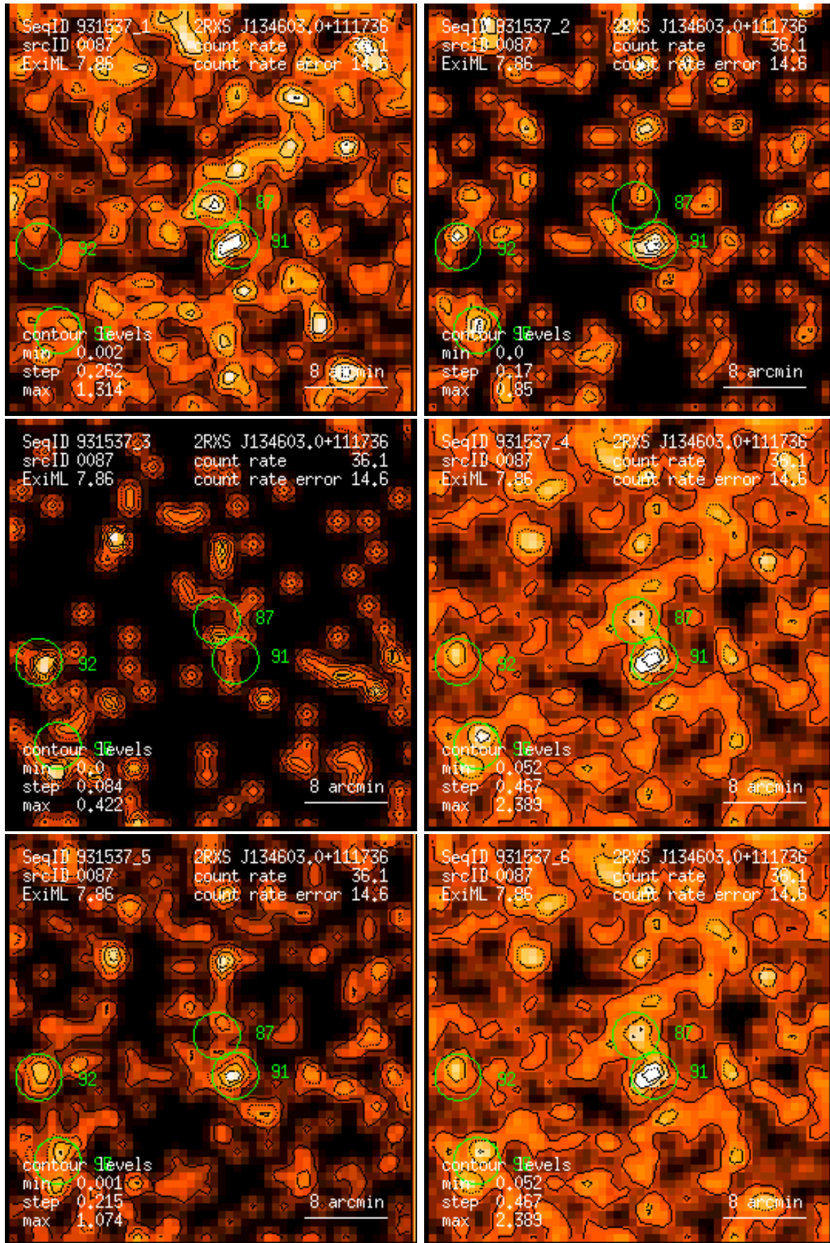
Figure 87: RASS 931537: detection 0087: band rate images, Gaussian filter: (1) PSPC channels 11 – 41, (2) 52 – 90, (3) 91 – 201, (4) 11 – 235, (5) 52 – 201, (6) 11 – 201. Broad band rates in counts/ks. Band rate contour levels in counts/ks/arcmin 2 .
