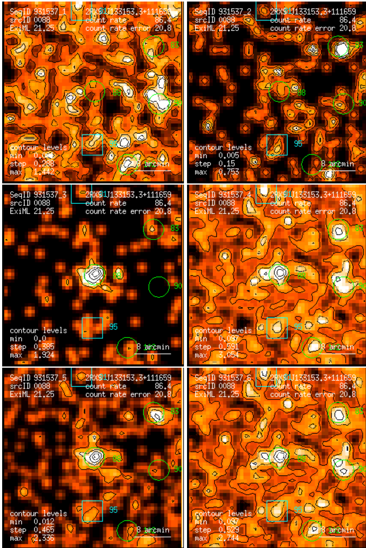
Figure 88: RASS 931537: detection 0088: band rate images, Gaussian filter: (1) PSPC channels 11 – 41, (2) 52 – 90, (3) 91 – 201, (4) 11 – 235, (5) 52 – 201, (6) 11 – 201. Broad band rates in counts/ks. Band rate contour levels in counts/ks/arcmin 2 .
