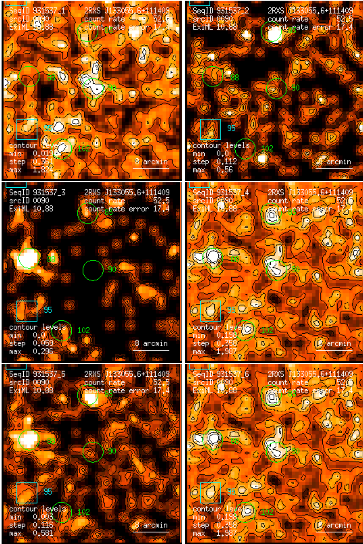
Figure 90: RASS 931537: detection 0090: band rate images, Gaussian filter: (1) PSPC channels 11 – 41, (2) 52 – 90, (3) 91 – 201, (4) 11 – 235, (5) 52 – 201, (6) 11 – 201. Broad band rates in counts/ks. Band rate contour levels in counts/ks/arcmin 2 .
