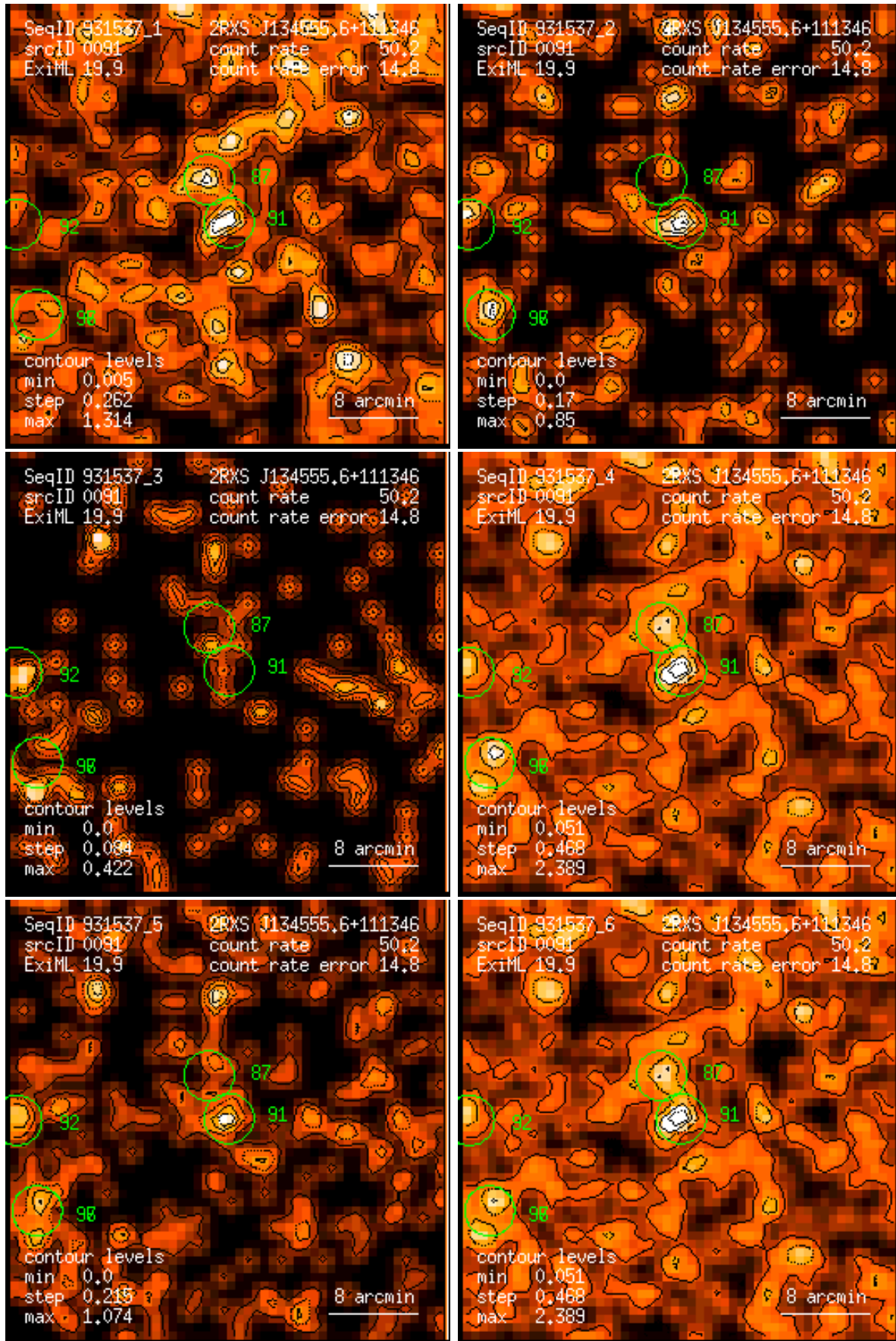
Figure 91: RASS 931537: detection 0091: band rate images, Gaussian filter: (1) PSPC channels 11 – 41, (2) 52 – 90, (3) 91 – 201, (4) 11 – 235, (5) 52 – 201, (6) 11 – 201. Broad band rates in counts/ks. Band rate contour levels in counts/ks/arcmin 2 .
