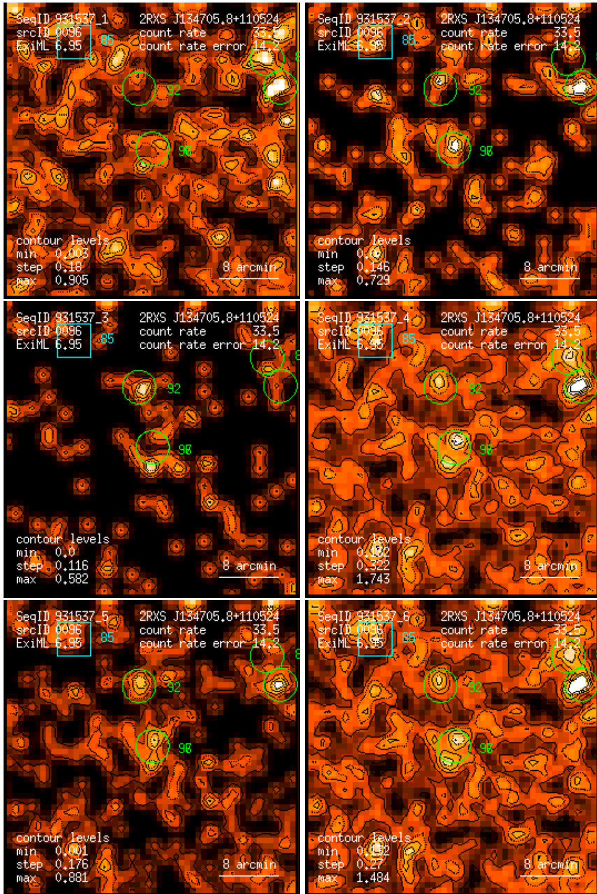
Figure 96: RASS 931537: detection 0096: band rate images, Gaussian filter: (1) PSPC channels 11 – 41, (2) 52 – 90, (3) 91 – 201, (4) 11 – 235, (5) 52 – 201, (6) 11 – 201. Broad band rates in counts/ks. Band rate contour levels in counts/ks/arcmin 2 .
