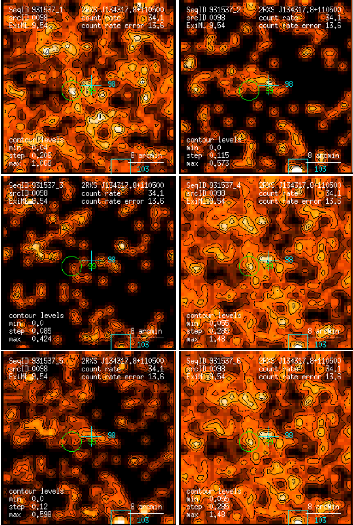
Figure 98: RASS 931537: detection 0098: band rate images, Gaussian filter: (1) PSPC channels 11 – 41, (2) 52 – 90, (3) 91 – 201, (4) 11 – 235, (5) 52 – 201, (6) 11 – 201. Broad band rates in counts/ks. Band rate contour levels in counts/ks/arcmin 2 .
