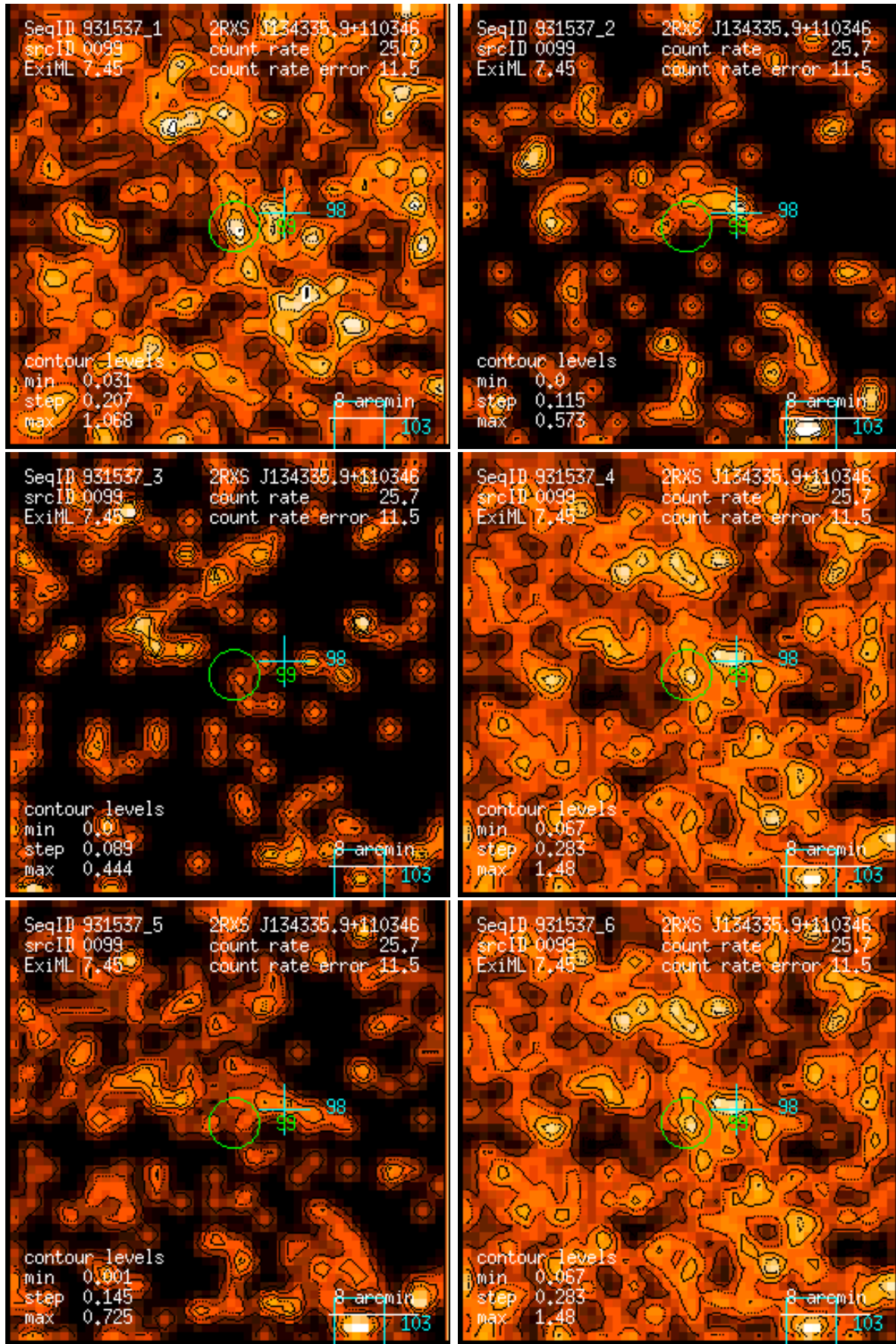
Figure 99: RASS 931537: detection 0099: band rate images, Gaussian filter: (1) PSPC channels 11 – 41, (2) 52 – 90, (3) 91 – 201, (4) 11 – 235, (5) 52 – 201, (6) 11 – 201. Broad band rates in counts/ks. Band rate contour levels in counts/ks/arcmin 2 .
