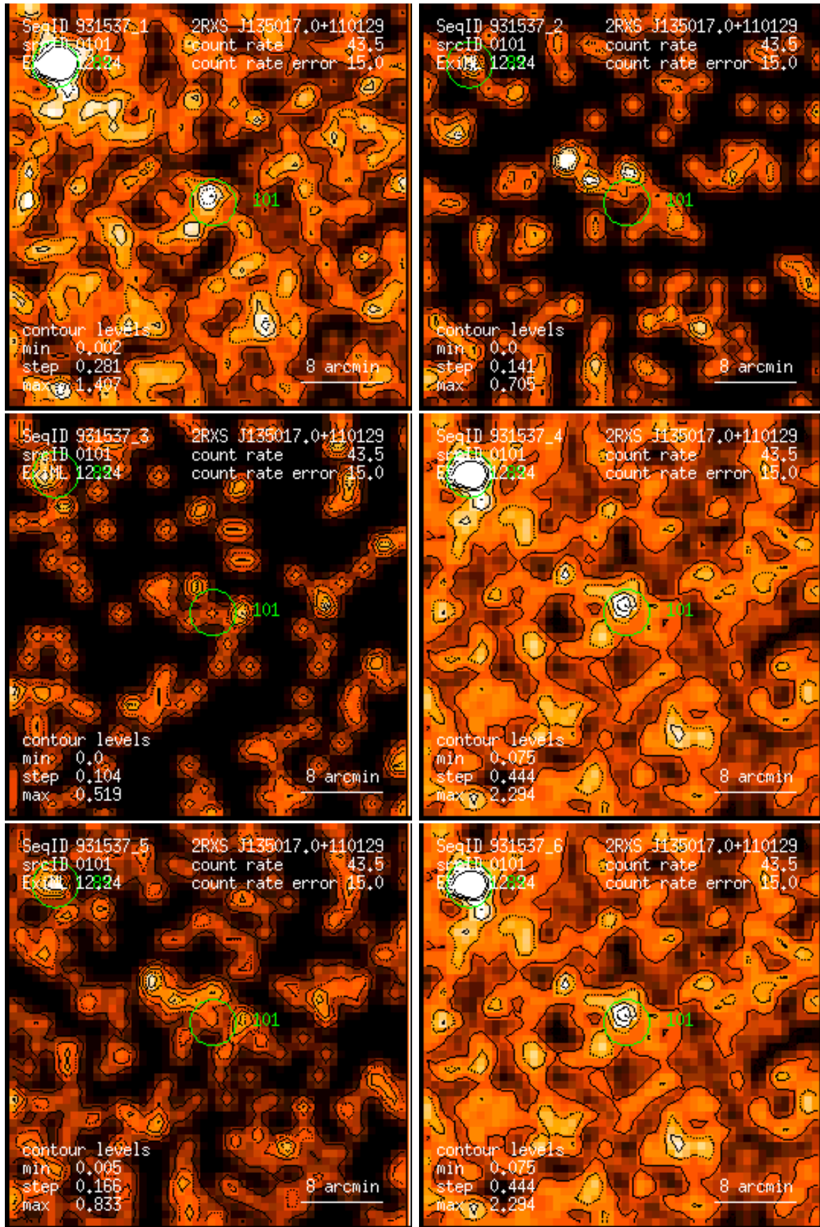
Figure 101: RASS 931537: detection 0101: band rate images, Gaussian filter: (1) PSPC channels 11 – 41, (2) 52 – 90, (3) 91 – 201, (4) 11 – 235, (5) 52 – 201, (6) 11 – 201. Broad band rates in counts/ks. Band rate contour levels in counts/ks/arcmin 2 .
