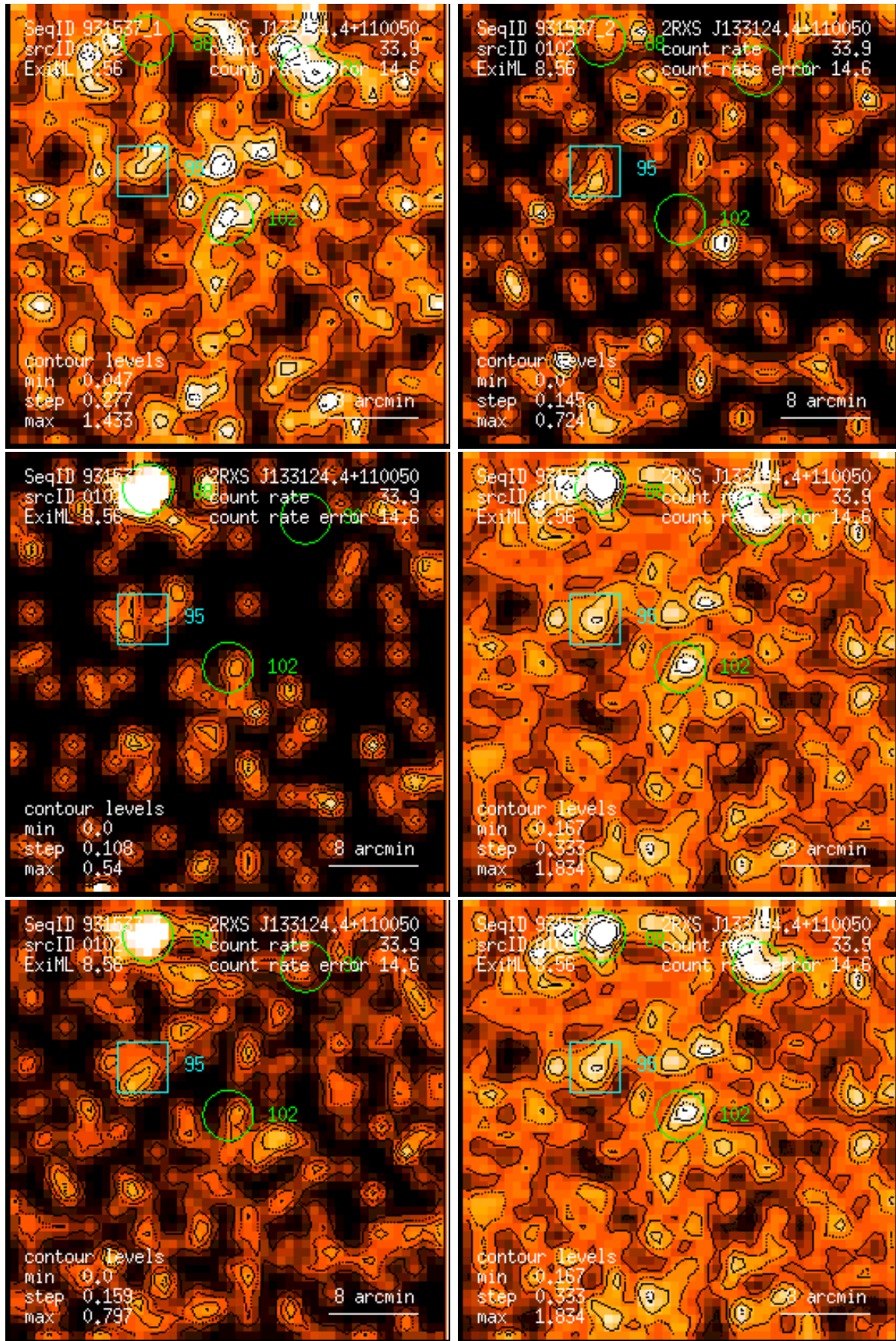
Figure 102: RASS 931537: detection 0102: band rate images, Gaussian filter: (1) PSPC channels 11 – 41, (2) 52 – 90, (3) 91 – 201, (4) 11 – 235, (5) 52 – 201, (6) 11 – 201. Broad band rates in counts/ks. Band rate contour levels in counts/ks/arcmin 2 .
