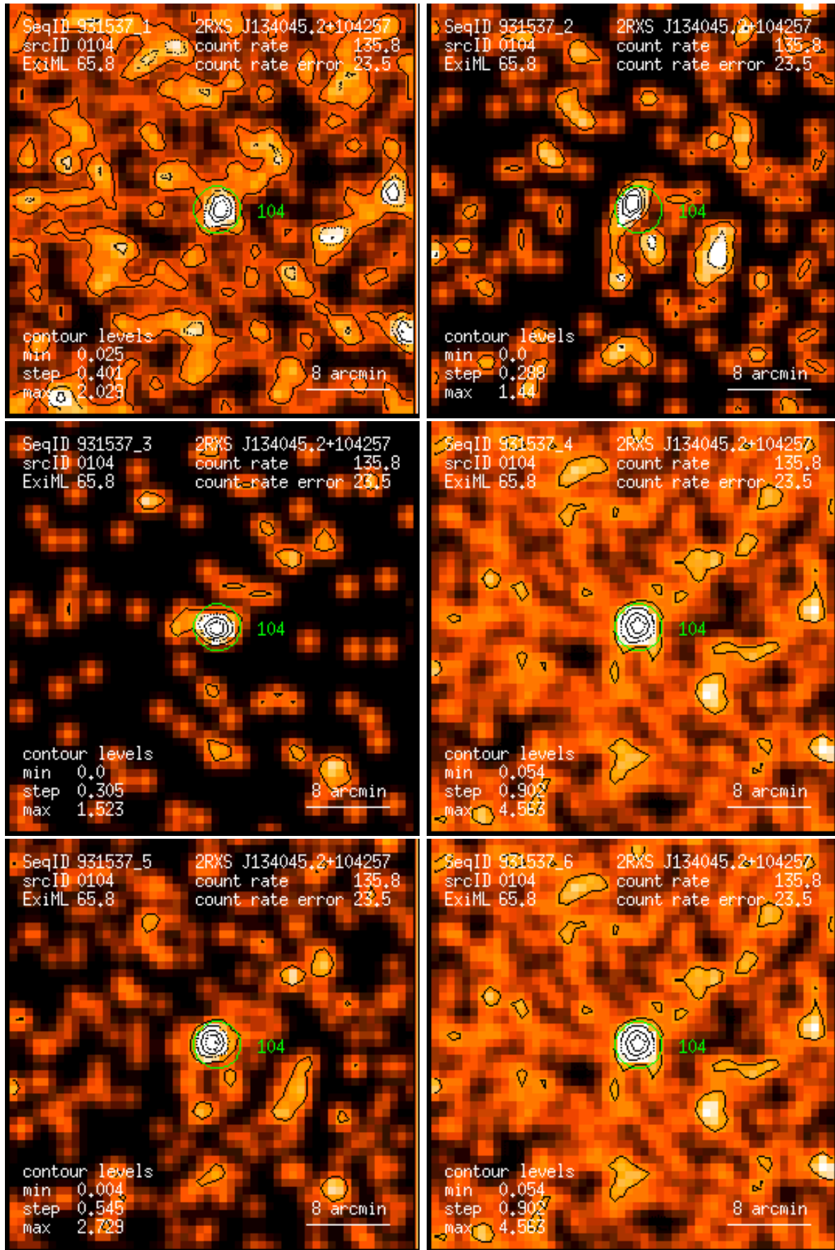
Figure 104: RASS 931537: detection 0104: band rate images, Gaussian filter: (1) PSPC channels 11 – 41, (2) 52 – 90, (3) 91 – 201, (4) 11 – 235, (5) 52 – 201, (6) 11 – 201. Broad band rates in counts/ks. Band rate contour levels in counts/ks/arcmin 2 .
