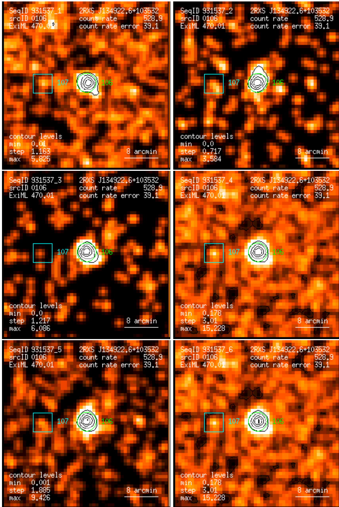
Figure 106: RASS 931537: detection 0106: band rate images, Gaussian filter: (1) PSPC channels 11 – 41, (2) 52 – 90, (3) 91 – 201, (4) 11 – 235, (5) 52 – 201, (6) 11 – 201. Broad band rates in counts/ks. Band rate contour levels in counts/ks/arcmin 2 .
