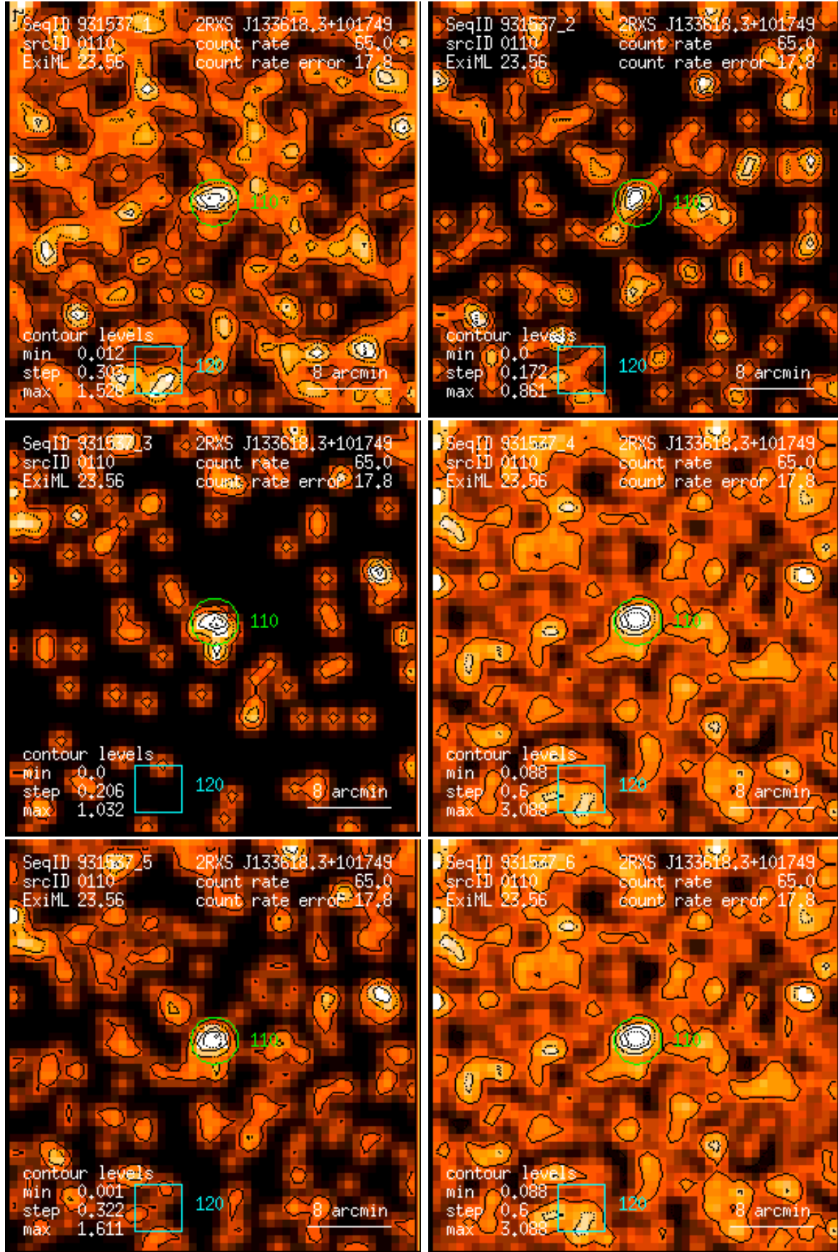
Figure 110: RASS 931537: detection 0110: band rate images, Gaussian filter: (1) PSPC channels 11 – 41, (2) 52 – 90, (3) 91 – 201, (4) 11 – 235, (5) 52 – 201, (6) 11 – 201. Broad band rates in counts/ks. Band rate contour levels in counts/ks/arcmin 2 .
