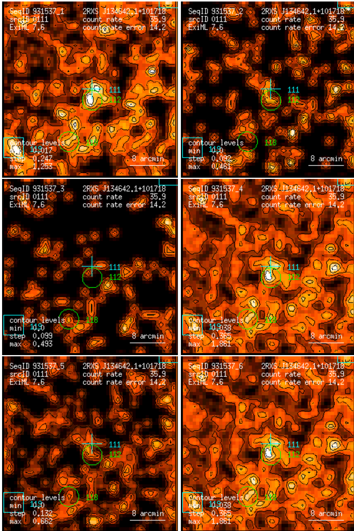
Figure 111: RASS 931537: detection 0111: band rate images, Gaussian filter: (1) PSPC channels 11 – 41, (2) 52 – 90, (3) 91 – 201, (4) 11 – 235, (5) 52 – 201, (6) 11 – 201. Broad band rates in counts/ks. Band rate contour levels in counts/ks/arcmin 2 .
