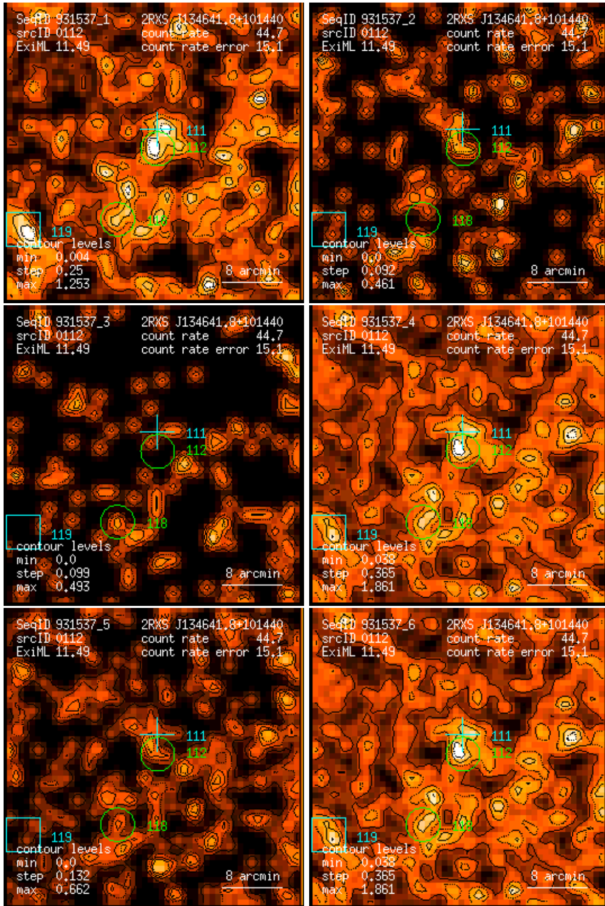
Figure 112: RASS 931537: detection 0112: band rate images, Gaussian filter: (1) PSPC channels 11 – 41, (2) 52 – 90, (3) 91 – 201, (4) 11 – 235, (5) 52 – 201, (6) 11 – 201. Broad band rates in counts/ks. Band rate contour levels in counts/ks/arcmin 2 .
