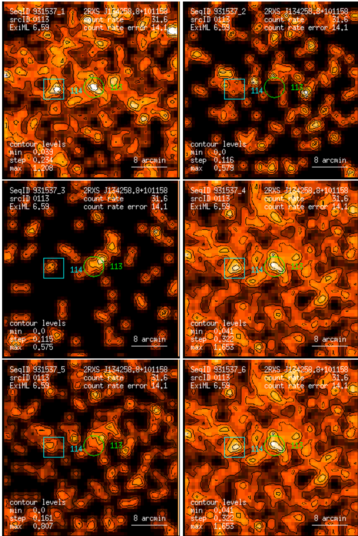
Figure 113: RASS 931537: detection 0113: band rate images, Gaussian filter: (1) PSPC channels 11 – 41, (2) 52 – 90, (3) 91 – 201, (4) 11 – 235, (5) 52 – 201, (6) 11 – 201. Broad band rates in counts/ks. Band rate contour levels in counts/ks/arcmin 2 .
