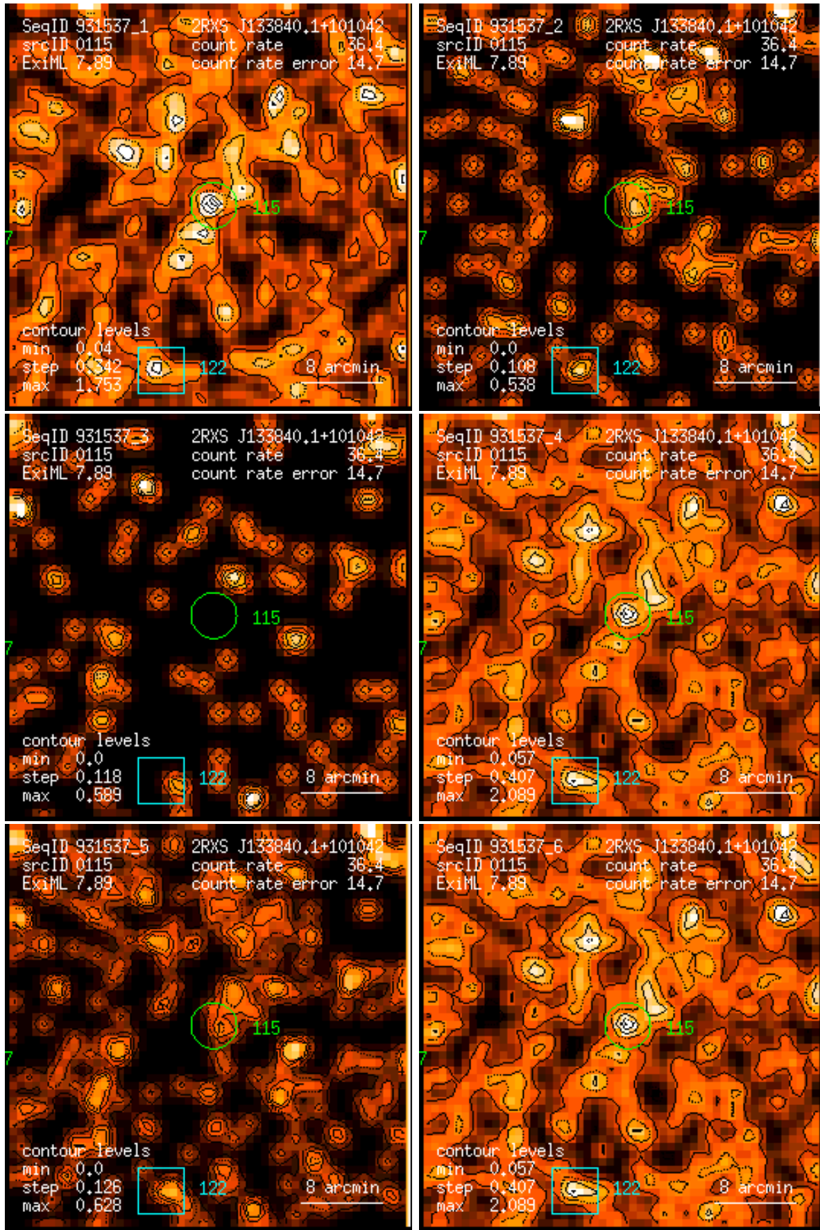
Figure 115: RASS 931537: detection 0115: band rate images, Gaussian filter: (1) PSPC channels 11 – 41, (2) 52 – 90, (3) 91 – 201, (4) 11 – 235, (5) 52 – 201, (6) 11 – 201. Broad band rates in counts/ks. Band rate contour levels in counts/ks/arcmin 2 .
