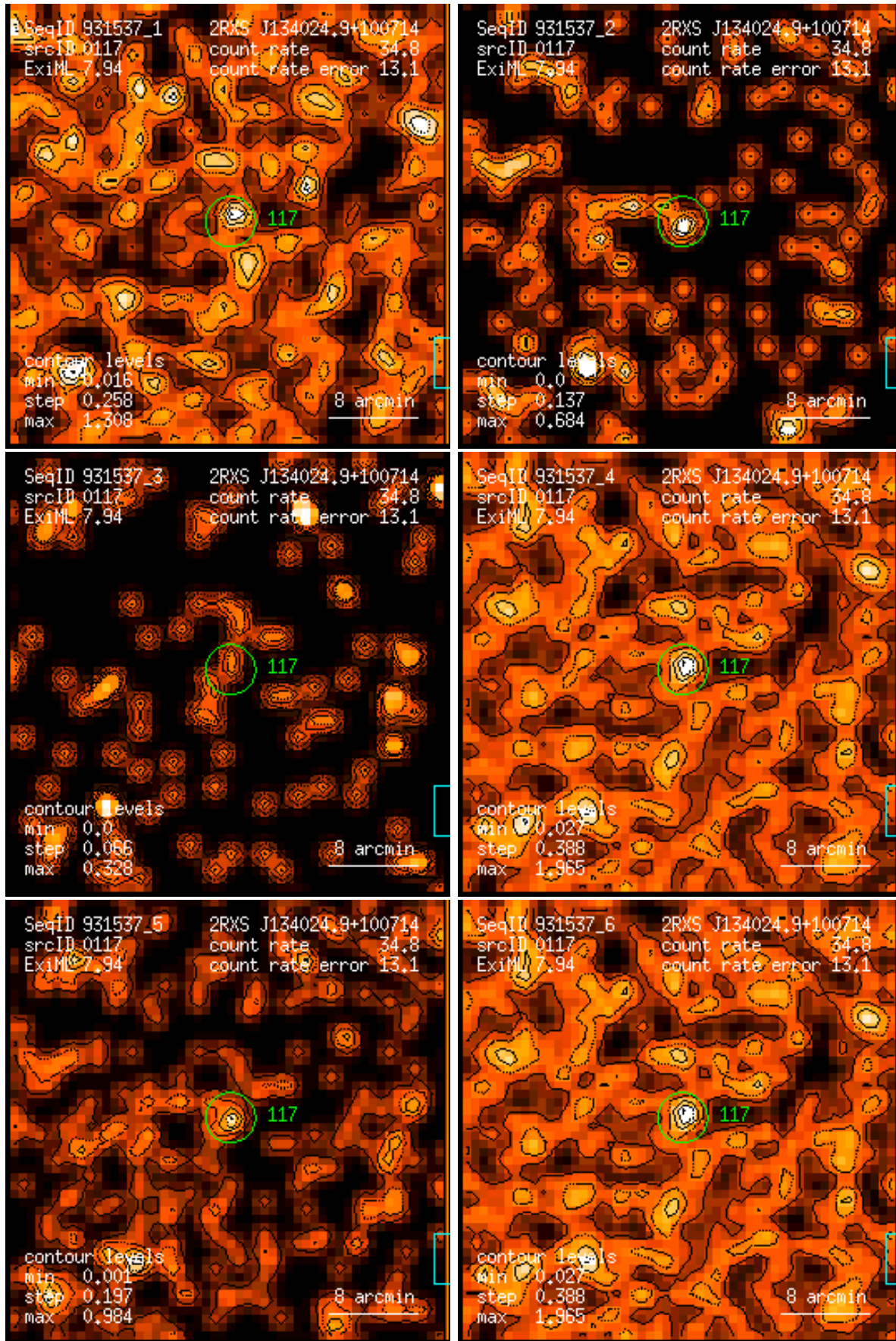
Figure 117: RASS 931537: detection 0117: band rate images, Gaussian filter: (1) PSPC channels 11 – 41, (2) 52 – 90, (3) 91 – 201, (4) 11 – 235, (5) 52 – 201, (6) 11 – 201. Broad band rates in counts/ks. Band rate contour levels in counts/ks/arcmin 2 .
