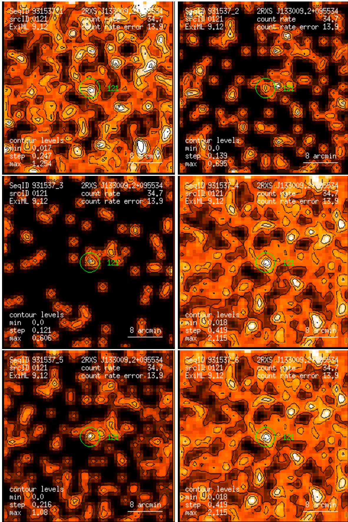
Figure 121: RASS 931537: detection 0121: band rate images, Gaussian filter: (1) PSPC channels 11 – 41, (2) 52 – 90, (3) 91 – 201, (4) 11 – 235, (5) 52 – 201, (6) 11 – 201. Broad band rates in counts/ks. Band rate contour levels in counts/ks/arcmin 2 .
