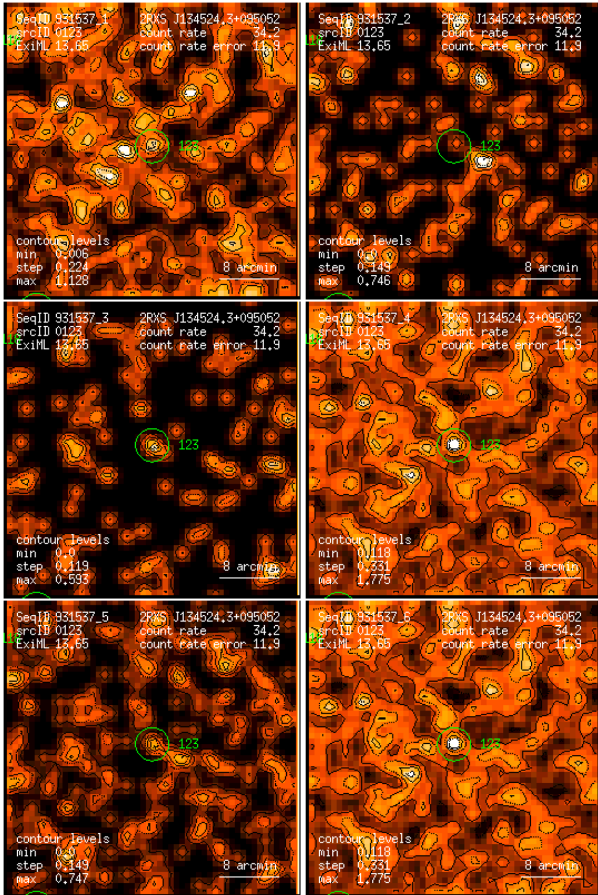
Figure 123: RASS 931537: detection 0123: band rate images, Gaussian filter: (1) PSPC channels 11 – 41, (2) 52 – 90, (3) 91 – 201, (4) 11 – 235, (5) 52 – 201, (6) 11 – 201. Broad band rates in counts/ks. Band rate contour levels in counts/ks/arcmin 2 .
