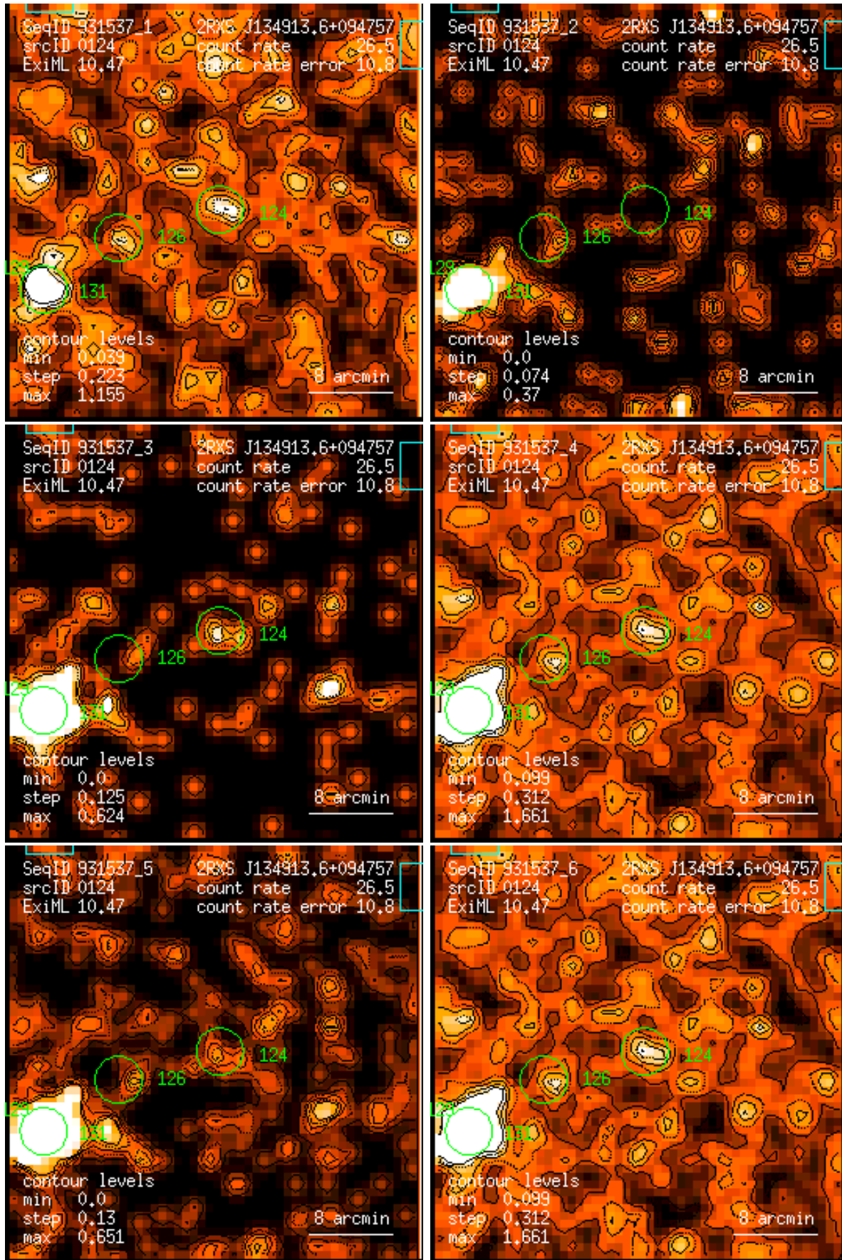
Figure 124: RASS 931537: detection 0124: band rate images, Gaussian filter: (1) PSPC channels 11 – 41, (2) 52 – 90, (3) 91 – 201, (4) 11 – 235, (5) 52 – 201, (6) 11 – 201. Broad band rates in counts/ks. Band rate contour levels in counts/ks/arcmin 2 .
