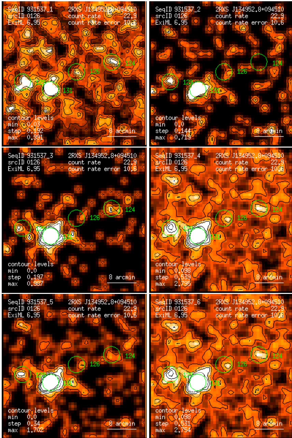
Figure 126: RASS 931537: detection 0126: band rate images, Gaussian filter: (1) PSPC channels 11 – 41, (2) 52 – 90, (3) 91 – 201, (4) 11 – 235, (5) 52 – 201, (6) 11 – 201. Broad band rates in counts/ks. Band rate contour levels in counts/ks/arcmin 2 .
