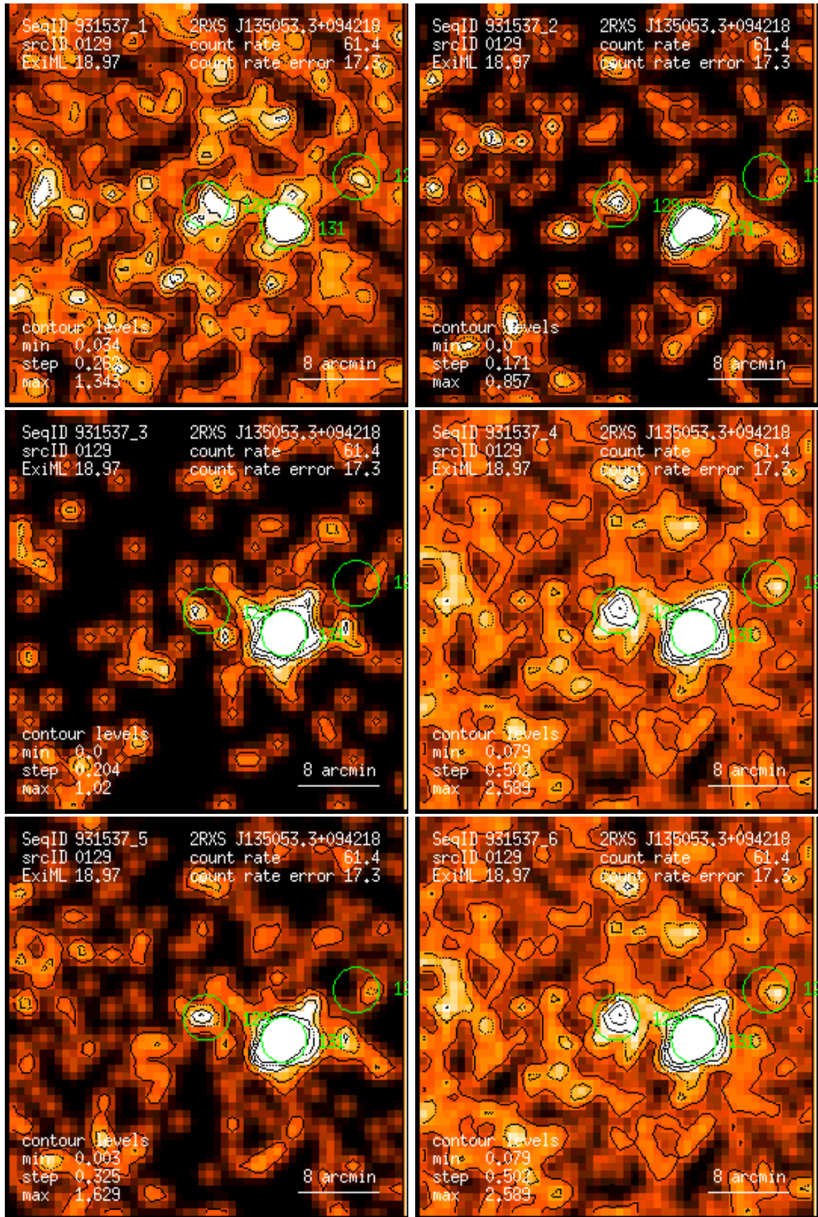
Figure 129: RASS 931537: detection 0129: band rate images, Gaussian filter: (1) PSPC channels 11 – 41, (2) 52 – 90, (3) 91 – 201, (4) 11 – 235, (5) 52 – 201, (6) 11 – 201. Broad band rates in counts/ks. Band rate contour levels in counts/ks/arcmin 2 .
