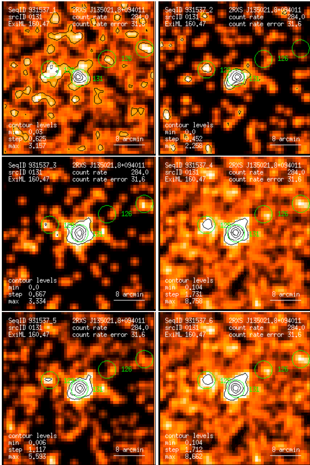
Figure 131: RASS 931537: detection 0131: band rate images, Gaussian filter: (1) PSPC channels 11 – 41, (2) 52 – 90, (3) 91 – 201, (4) 11 – 235, (5) 52 – 201, (6) 11 – 201. Broad band rates in counts/ks. Band rate contour levels in counts/ks/arcmin 2 .
