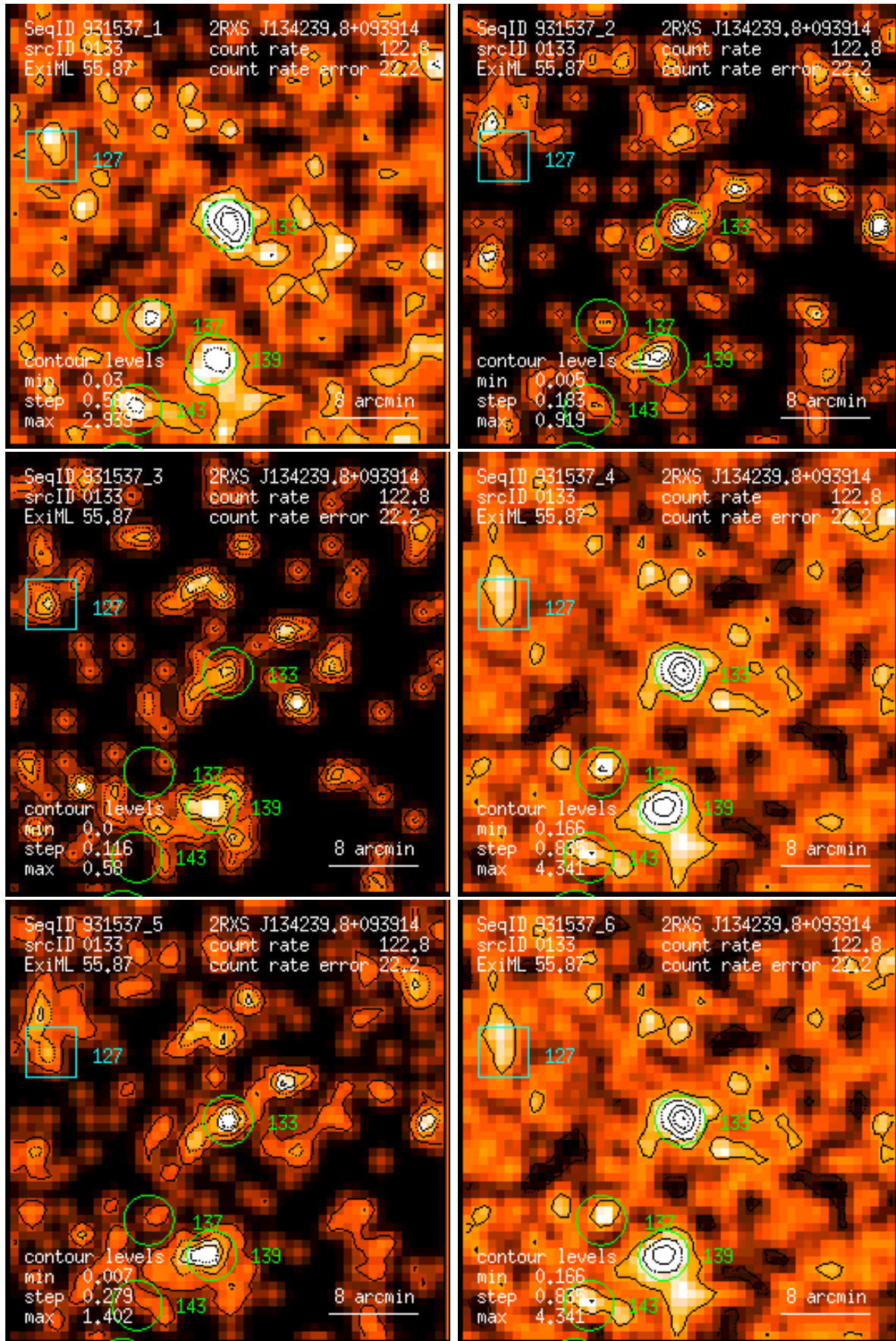
Figure 133: RASS 931537: detection 0133: band rate images, Gaussian filter: (1) PSPC channels 11 – 41, (2) 52 – 90, (3) 91 – 201, (4) 11 – 235, (5) 52 – 201, (6) 11 – 201. Broad band rates in counts/ks. Band rate contour levels in counts/ks/arcmin 2 .
