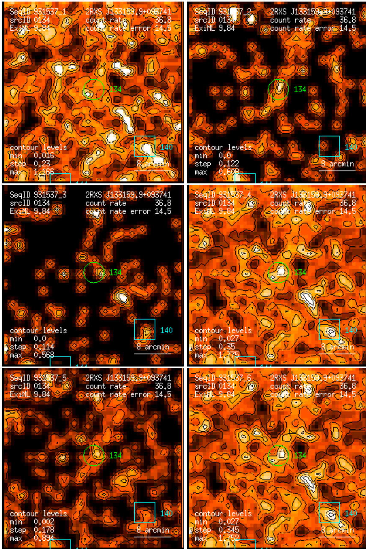
Figure 134: RASS 931537: detection 0134: band rate images, Gaussian filter: (1) PSPC channels 11 – 41, (2) 52 – 90, (3) 91 – 201, (4) 11 – 235, (5) 52 – 201, (6) 11 – 201. Broad band rates in counts/ks. Band rate contour levels in counts/ks/arcmin 2 .
