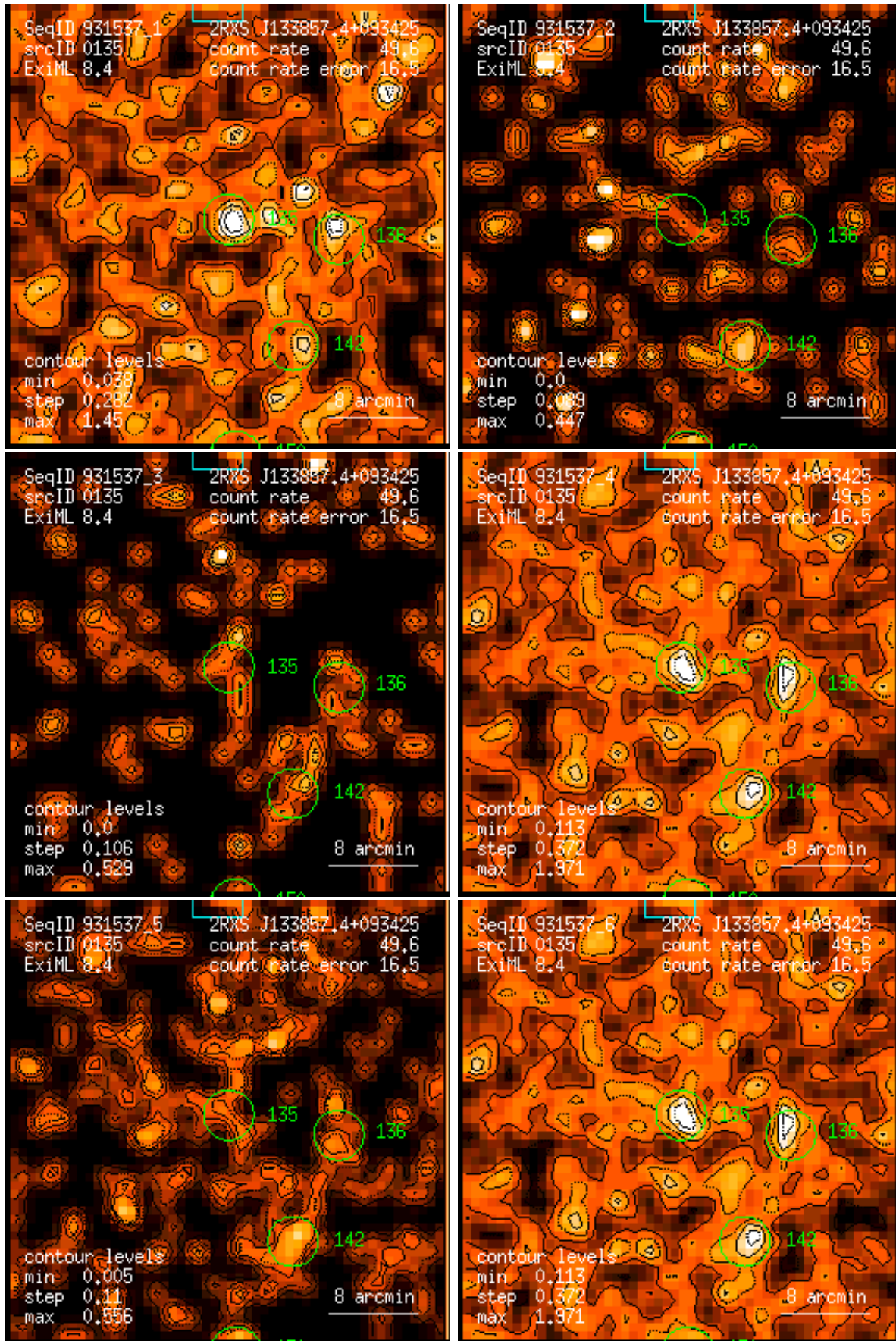
Figure 135: RASS 931537: detection 0135: band rate images, Gaussian filter: (1) PSPC channels 11 – 41, (2) 52 – 90, (3) 91 – 201, (4) 11 – 235, (5) 52 – 201, (6) 11 – 201. Broad band rates in counts/ks. Band rate contour levels in counts/ks/arcmin 2 .
