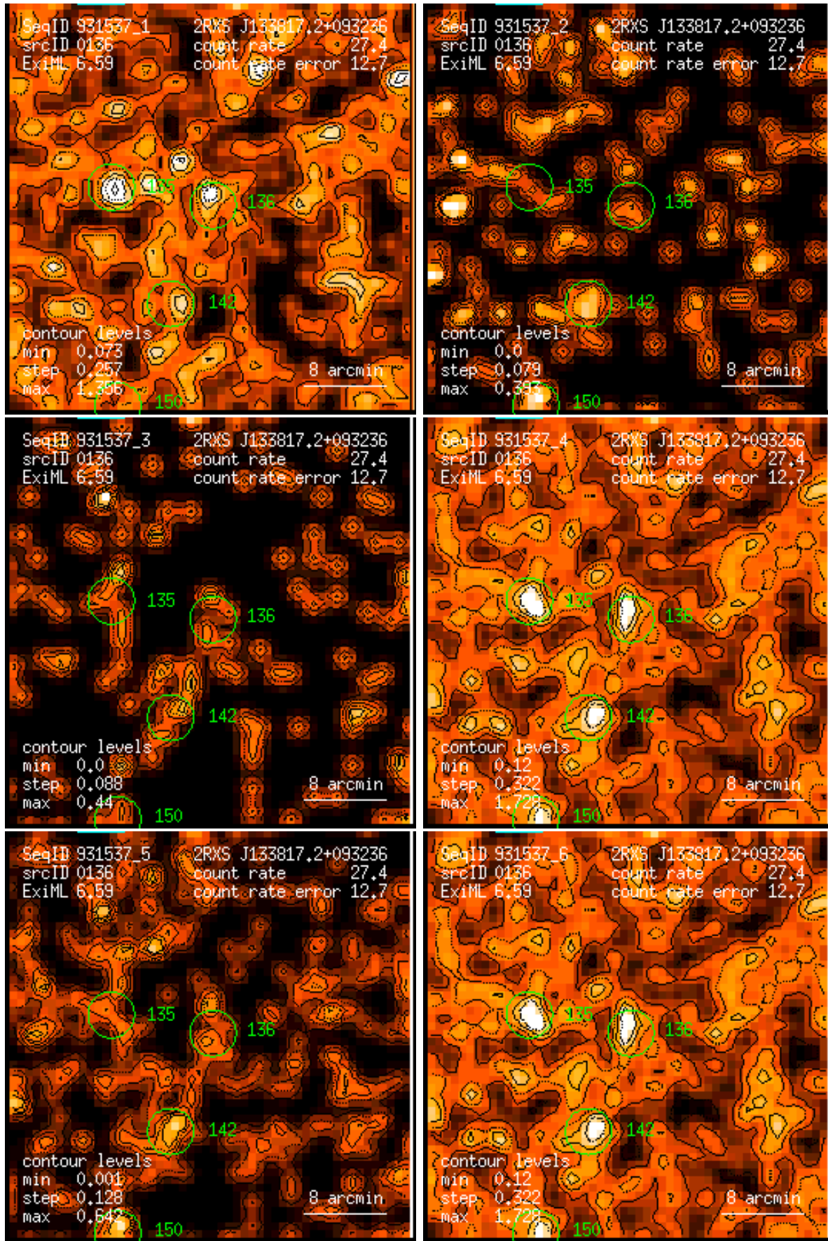
Figure 136: RASS 931537: detection 0136: band rate images, Gaussian filter: (1) PSPC channels 11 – 41, (2) 52 – 90, (3) 91 – 201, (4) 11 – 235, (5) 52 – 201, (6) 11 – 201. Broad band rates in counts/ks. Band rate contour levels in counts/ks/arcmin 2 .
