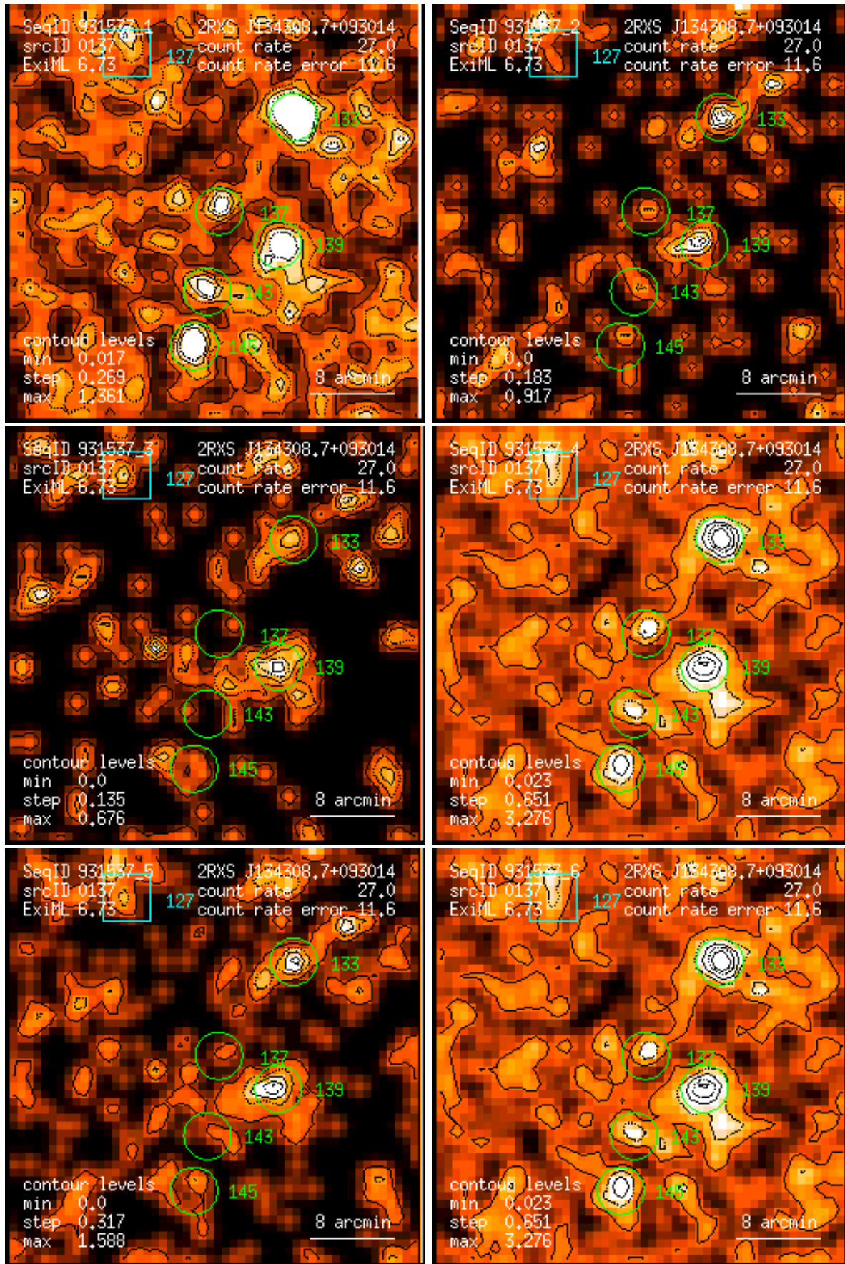
Figure 137: RASS 931537: detection 0137: band rate images, Gaussian filter: (1) PSPC channels 11 – 41, (2) 52 – 90, (3) 91 – 201, (4) 11 – 235, (5) 52 – 201, (6) 11 – 201. Broad band rates in counts/ks. Band rate contour levels in counts/ks/arcmin 2 .
