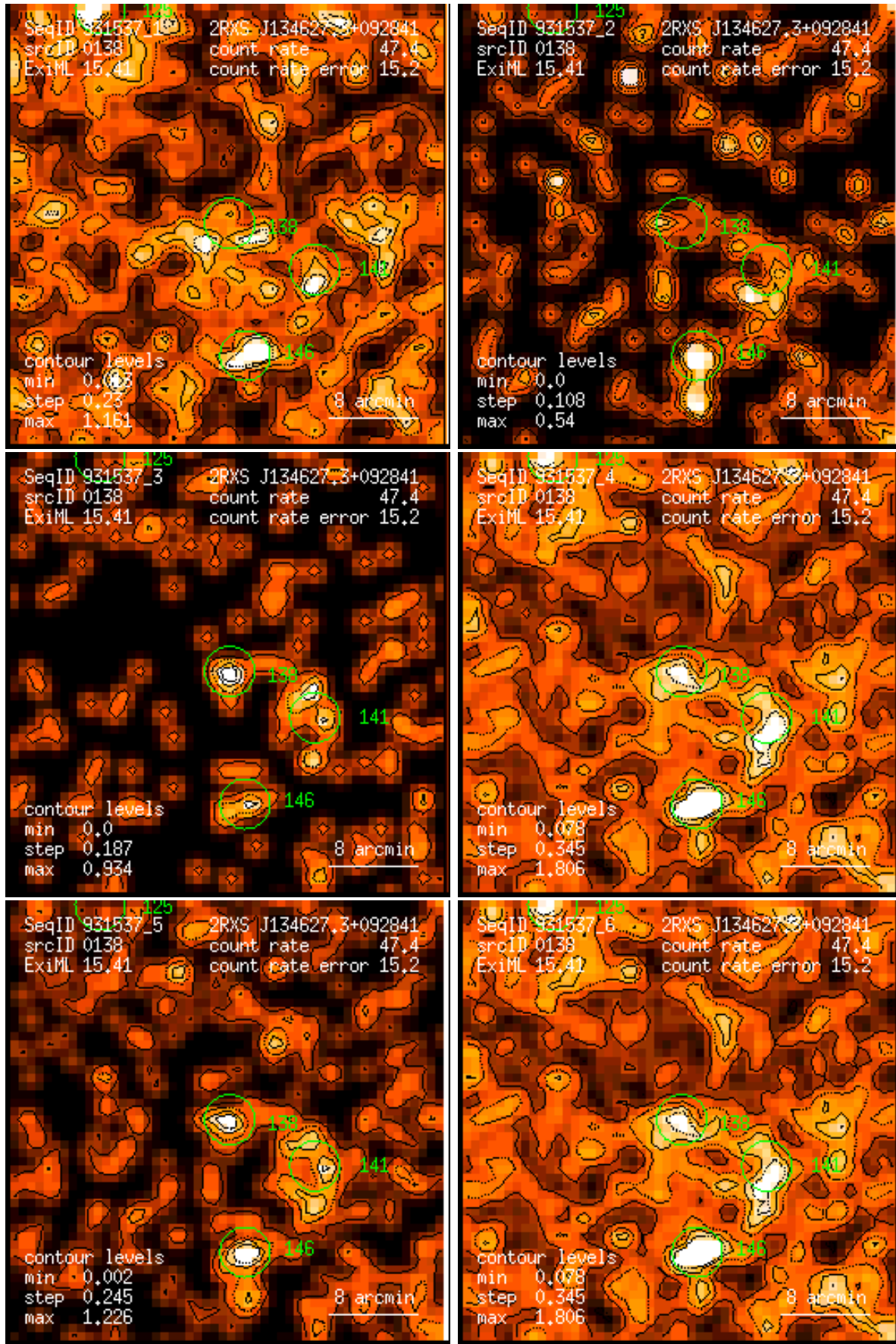
Figure 138: RASS 931537: detection 0138: band rate images, Gaussian filter: (1) PSPC channels 11 – 41, (2) 52 – 90, (3) 91 – 201, (4) 11 – 235, (5) 52 – 201, (6) 11 – 201. Broad band rates in counts/ks. Band rate contour levels in counts/ks/arcmin 2 .
