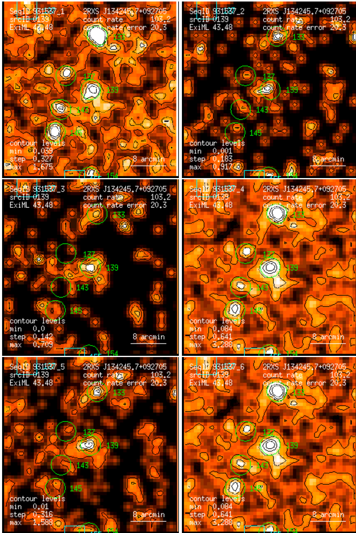
Figure 139: RASS 931537: detection 0139: band rate images, Gaussian filter: (1) PSPC channels 11 – 41, (2) 52 – 90, (3) 91 – 201, (4) 11 – 235, (5) 52 – 201, (6) 11 – 201. Broad band rates in counts/ks. Band rate contour levels in counts/ks/arcmin 2 .
