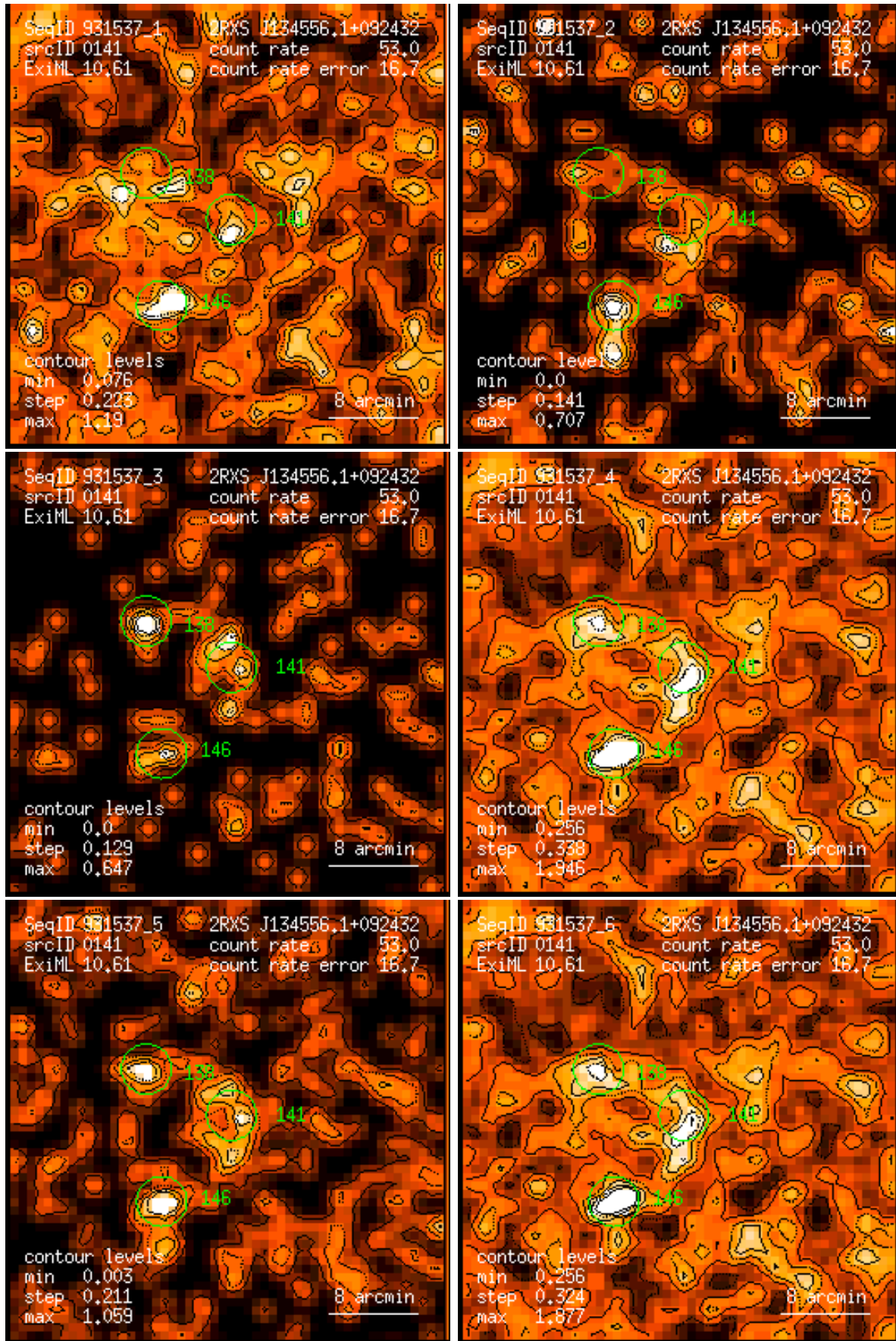
Figure 141: RASS 931537: detection 0141: band rate images, Gaussian filter: (1) PSPC channels 11 – 41, (2) 52 – 90, (3) 91 – 201, (4) 11 – 235, (5) 52 – 201, (6) 11 – 201. Broad band rates in counts/ks. Band rate contour levels in counts/ks/arcmin 2 .
