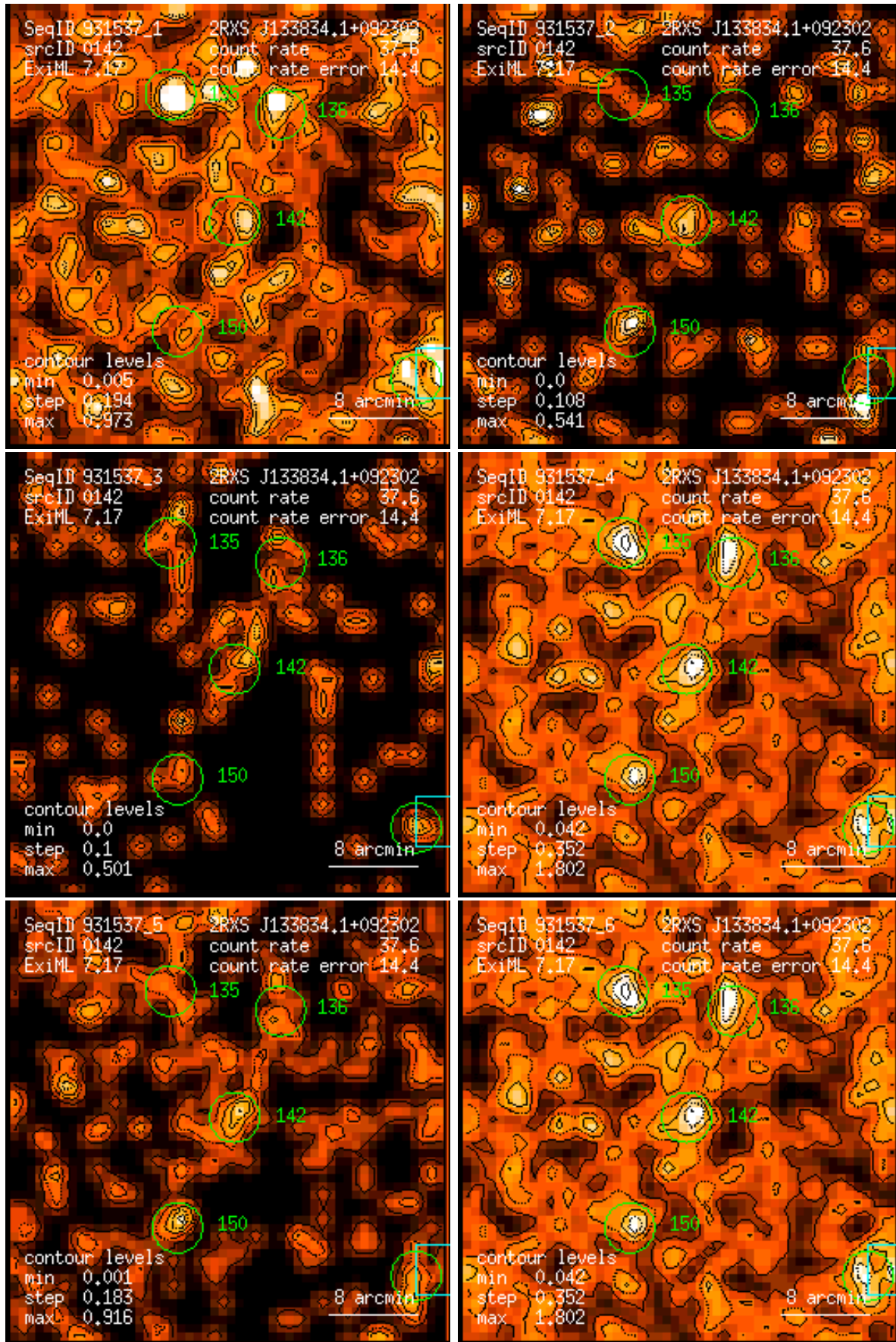
Figure 142: RASS 931537: detection 0142: band rate images, Gaussian filter: (1) PSPC channels 11 – 41, (2) 52 – 90, (3) 91 – 201, (4) 11 – 235, (5) 52 – 201, (6) 11 – 201. Broad band rates in counts/ks. Band rate contour levels in counts/ks/arcmin 2 .
