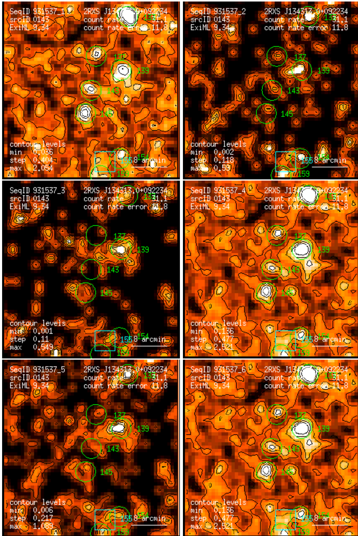
Figure 143: RASS 931537: detection 0143: band rate images, Gaussian filter: (1) PSPC channels 11 – 41, (2) 52 – 90, (3) 91 – 201, (4) 11 – 235, (5) 52 – 201, (6) 11 – 201. Broad band rates in counts/ks. Band rate contour levels in counts/ks/arcmin 2 .
