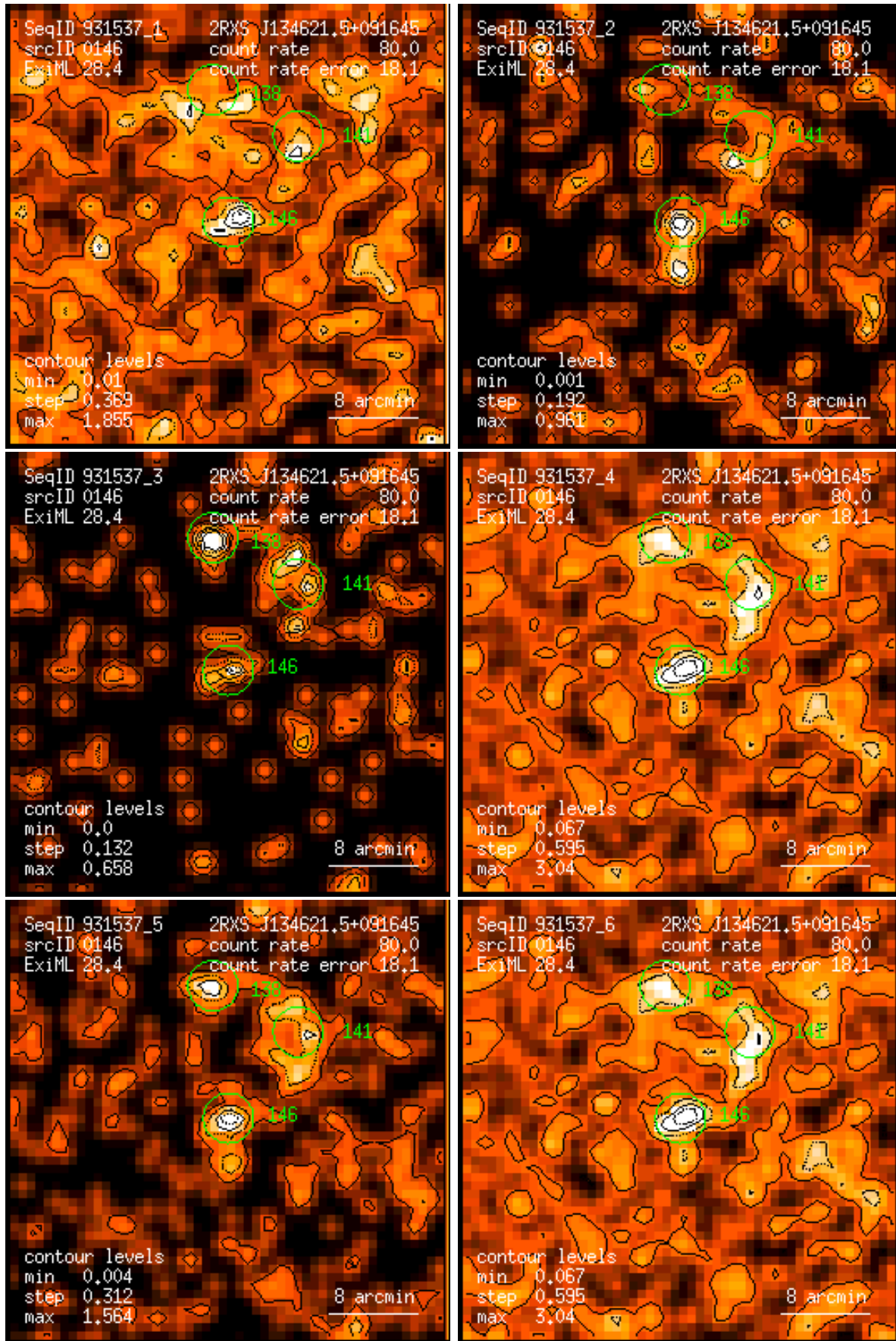
Figure 146: RASS 931537: detection 0146: band rate images, Gaussian filter: (1) PSPC channels 11 – 41, (2) 52 – 90, (3) 91 – 201, (4) 11 – 235, (5) 52 – 201, (6) 11 – 201. Broad band rates in counts/ks. Band rate contour levels in counts/ks/arcmin 2 .
