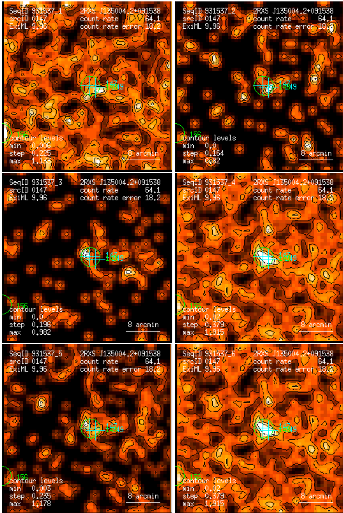
Figure 147: RASS 931537: detection 0147: band rate images, Gaussian filter: (1) PSPC channels 11 – 41, (2) 52 – 90, (3) 91 – 201, (4) 11 – 235, (5) 52 – 201, (6) 11 – 201. Broad band rates in counts/ks. Band rate contour levels in counts/ks/arcmin 2 .
