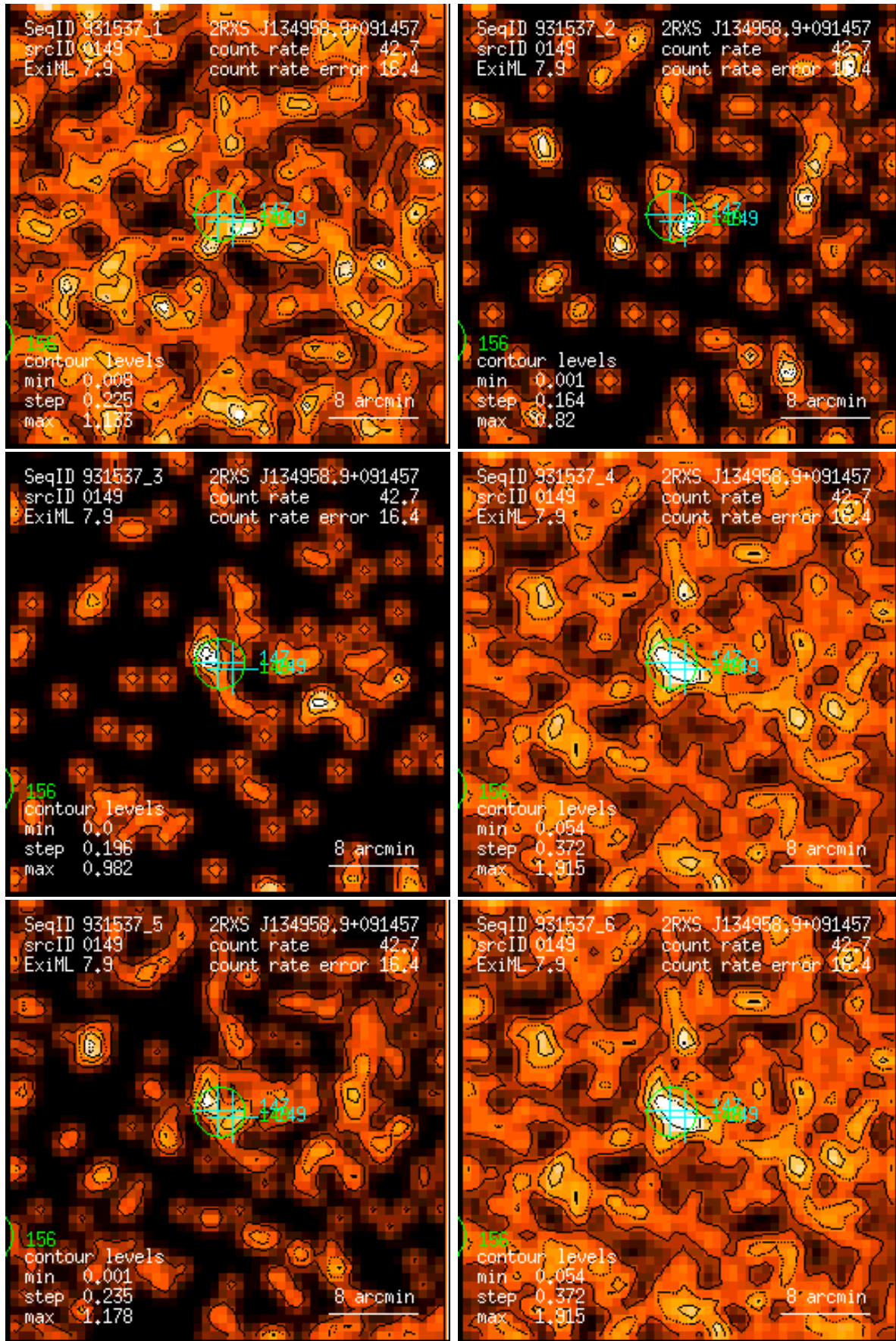
Figure 149: RASS 931537: detection 0149: band rate images, Gaussian filter: (1) PSPC channels 11 – 41, (2) 52 – 90, (3) 91 – 201, (4) 11 – 235, (5) 52 – 201, (6) 11 – 201. Broad band rates in counts/ks. Band rate contour levels in counts/ks/arcmin 2 .
