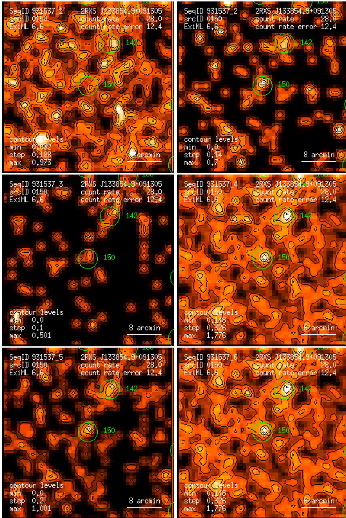
Figure 150: RASS 931537: detection 0150: band rate images, Gaussian filter: (1) PSPC channels 11 – 41, (2) 52 – 90, (3) 91 – 201, (4) 11 – 235, (5) 52 – 201, (6) 11 – 201. Broad band rates in counts/ks. Band rate contour levels in counts/ks/arcmin 2 .
