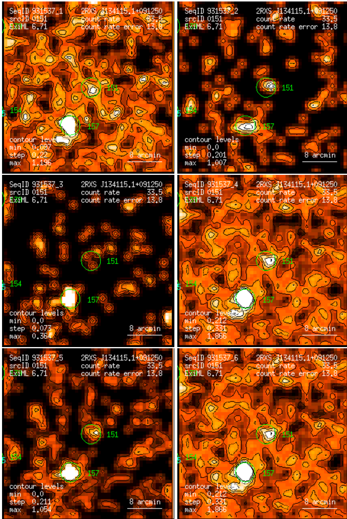
Figure 151: RASS 931537: detection 0151: band rate images, Gaussian filter: (1) PSPC channels 11 – 41, (2) 52 – 90, (3) 91 – 201, (4) 11 – 235, (5) 52 – 201, (6) 11 – 201. Broad band rates in counts/ks. Band rate contour levels in counts/ks/arcmin 2 .
