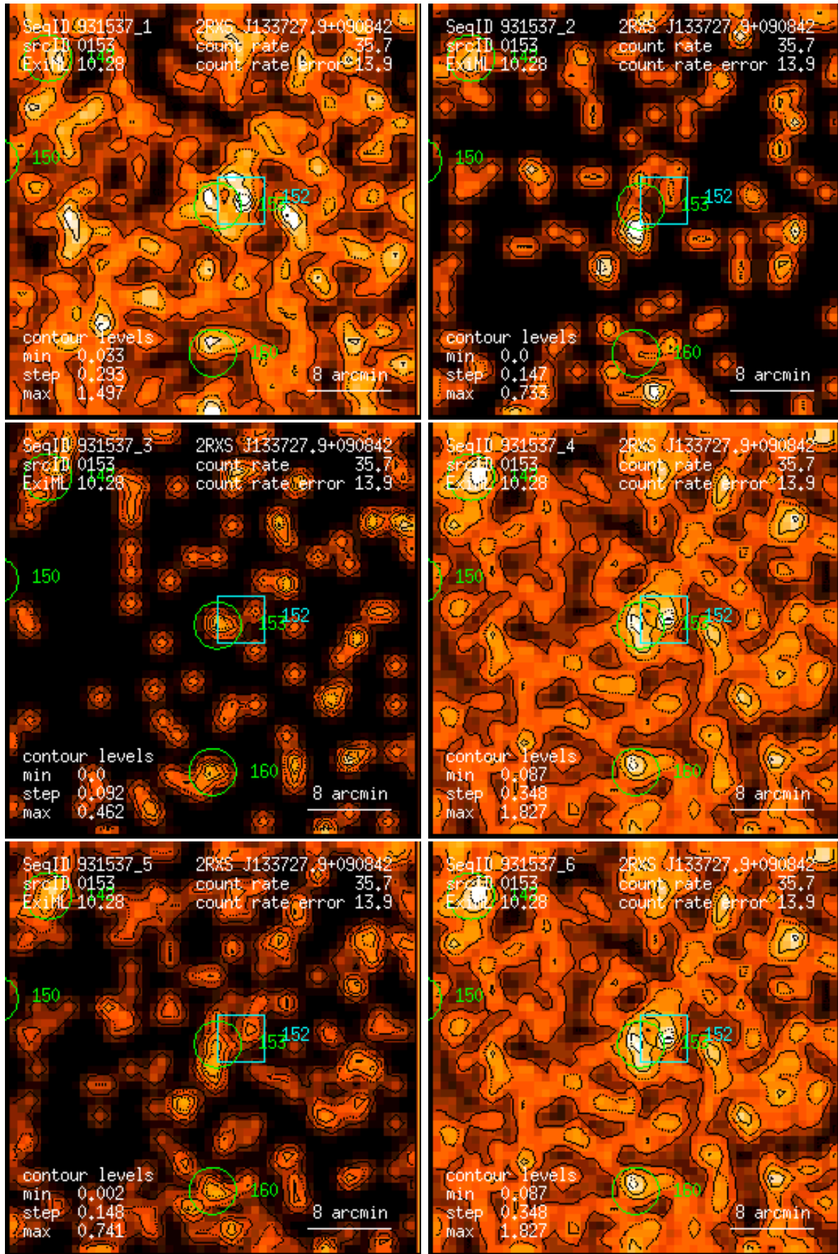
Figure 153: RASS 931537: detection 0153: band rate images, Gaussian filter: (1) PSPC channels 11 – 41, (2) 52 – 90, (3) 91 – 201, (4) 11 – 235, (5) 52 – 201, (6) 11 – 201. Broad band rates in counts/ks. Band rate contour levels in counts/ks/arcmin 2 .
