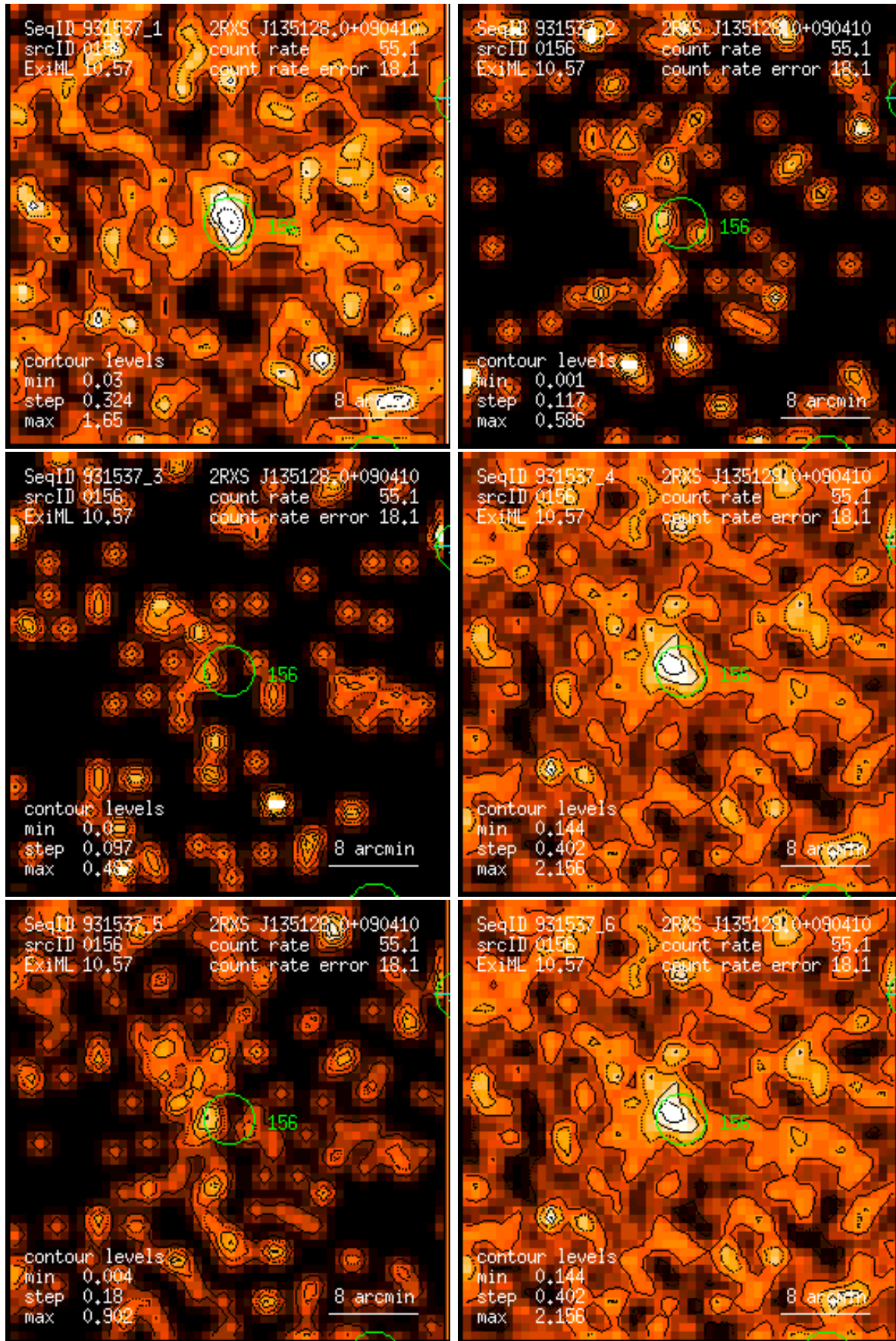
Figure 156: RASS 931537: detection 0156: band rate images, Gaussian filter: (1) PSPC channels 11 – 41, (2) 52 – 90, (3) 91 – 201, (4) 11 – 235, (5) 52 – 201, (6) 11 – 201. Broad band rates in counts/ks. Band rate contour levels in counts/ks/arcmin 2 .
