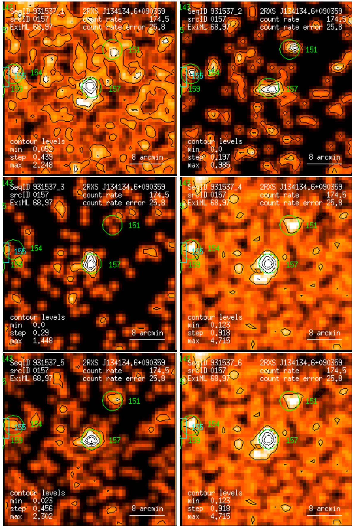
Figure 157: RASS 931537: detection 0157: band rate images, Gaussian filter: (1) PSPC channels 11 – 41, (2) 52 – 90, (3) 91 – 201, (4) 11 – 235, (5) 52 – 201, (6) 11 – 201. Broad band rates in counts/ks. Band rate contour levels in counts/ks/arcmin 2 .
