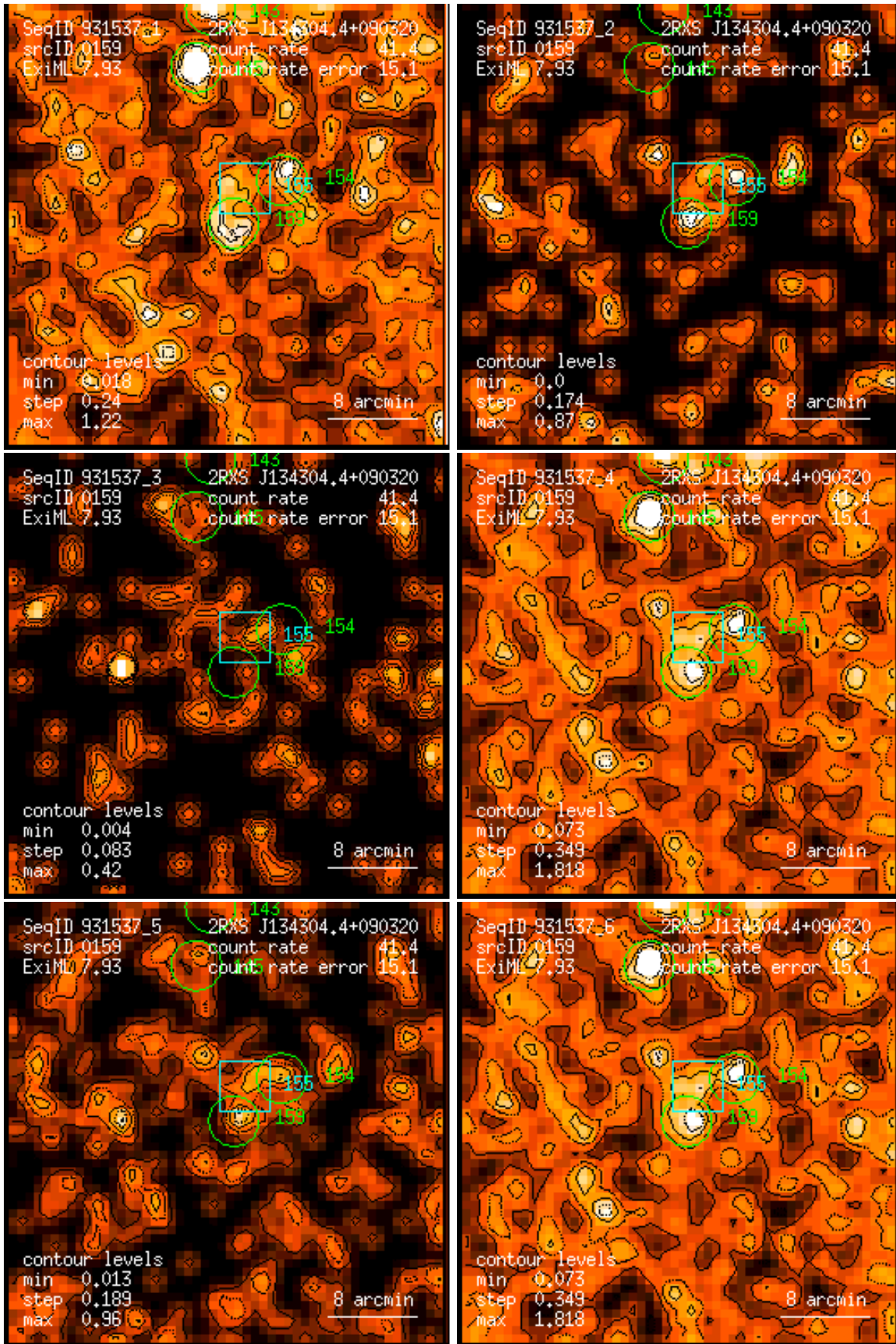
Figure 159: RASS 931537: detection 0159: band rate images, Gaussian filter: (1) PSPC channels 11 – 41, (2) 52 – 90, (3) 91 – 201, (4) 11 – 235, (5) 52 – 201, (6) 11 – 201. Broad band rates in counts/ks. Band rate contour levels in counts/ks/arcmin 2 .
