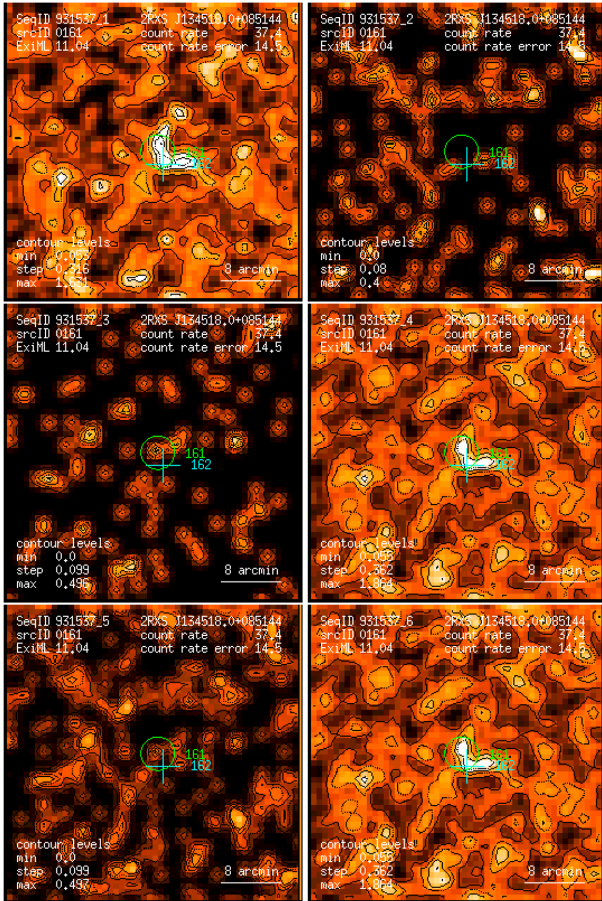
Figure 161: RASS 931537: detection 0161: band rate images, Gaussian filter: (1) PSPC channels 11 – 41, (2) 52 – 90, (3) 91 – 201, (4) 11 – 235, (5) 52 – 201, (6) 11 – 201. Broad band rates in counts/ks. Band rate contour levels in counts/ks/arcmin 2 .
