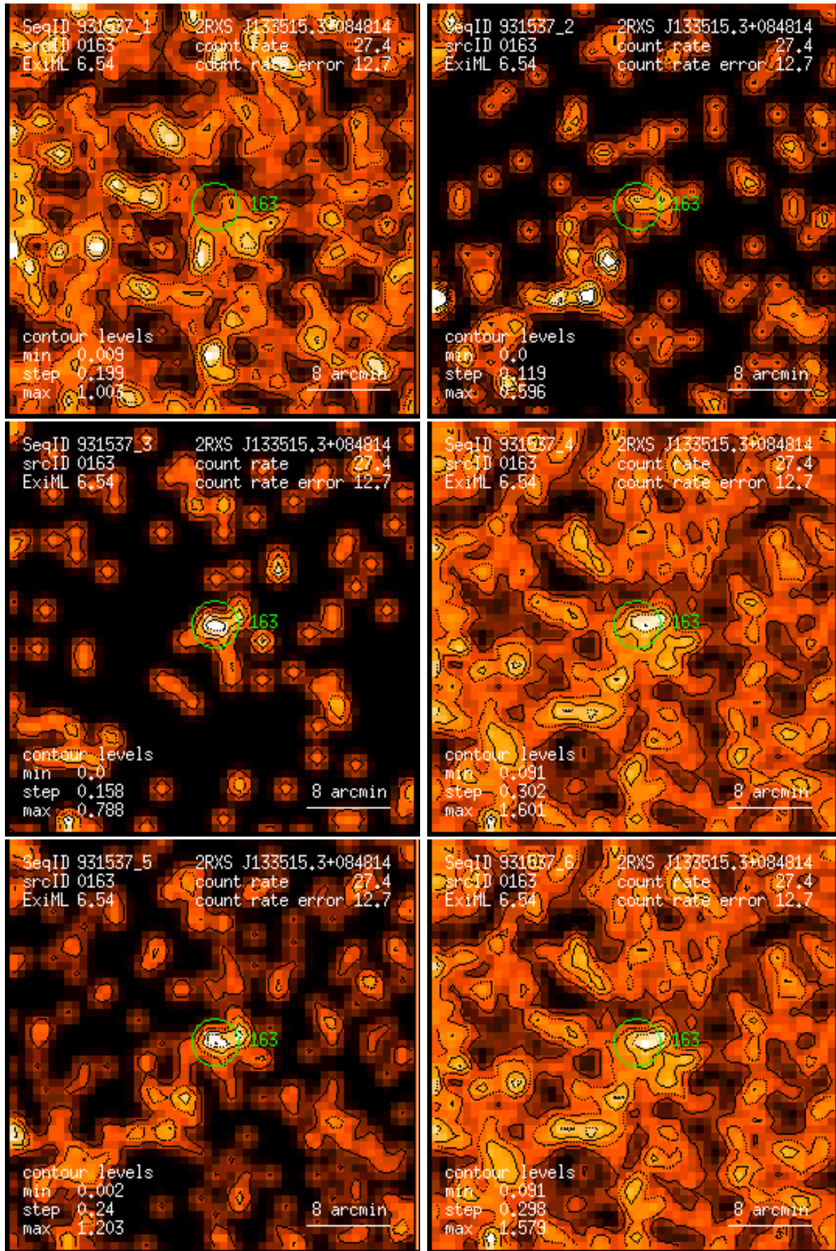
Figure 163: RASS 931537: detection 0163: band rate images, Gaussian filter: (1) PSPC channels 11 – 41, (2) 52 – 90, (3) 91 – 201, (4) 11 – 235, (5) 52 – 201, (6) 11 – 201. Broad band rates in counts/ks. Band rate contour levels in counts/ks/arcmin 2 .
