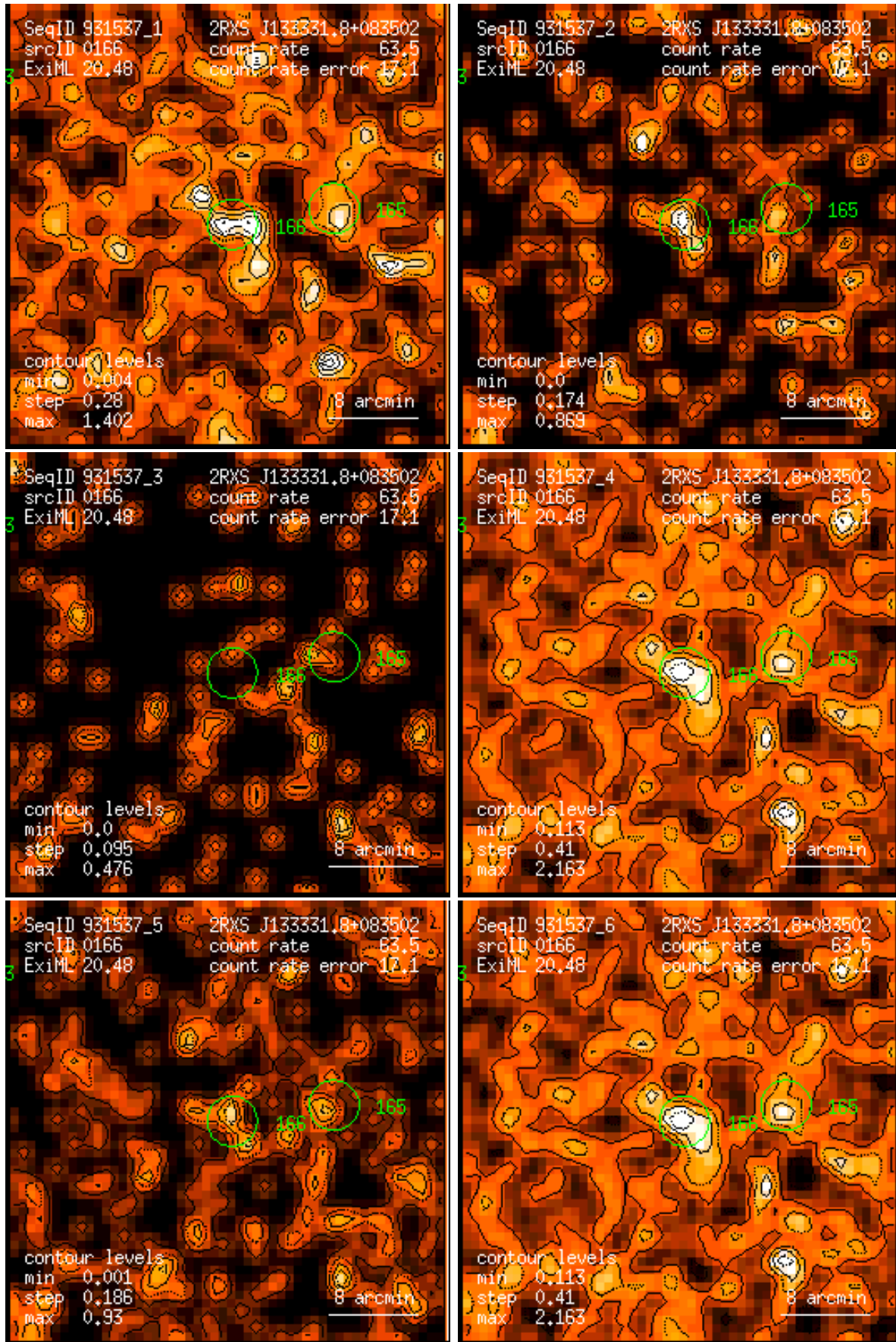
Figure 166: RASS 931537: detection 0166: band rate images, Gaussian filter: (1) PSPC channels 11 – 41, (2) 52 – 90, (3) 91 – 201, (4) 11 – 235, (5) 52 – 201, (6) 11 – 201. Broad band rates in counts/ks. Band rate contour levels in counts/ks/arcmin 2 .
